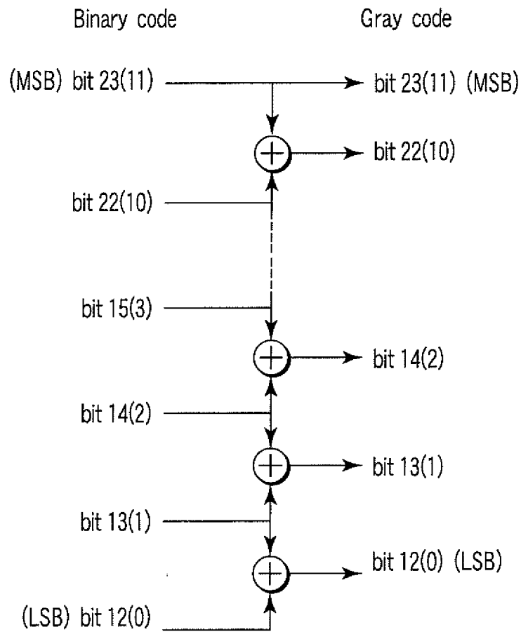
Explanatory diagram of Gray code conversion algorithm
