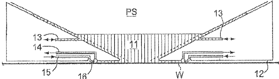
Fig. 5 (Prior Art)
