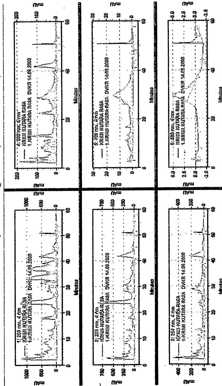
Figure 7 CHROMATOGRAMS OF A HERBAL FORMULATION KRIMIKUTARA RAS AT DIFFERENT WAVELENGTHS (The existing method)
