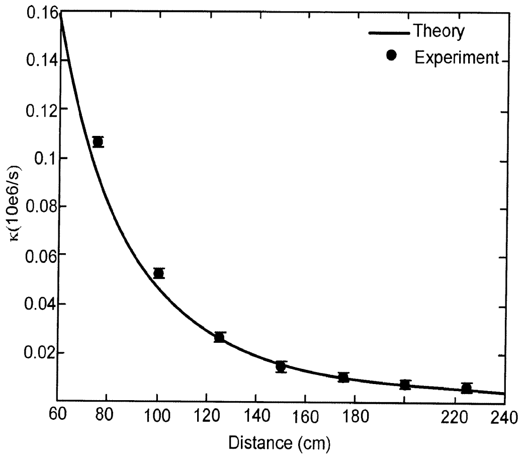
Comparison of experimental and theoretical values for \kappa as a function of the separation between the source and device coils.
