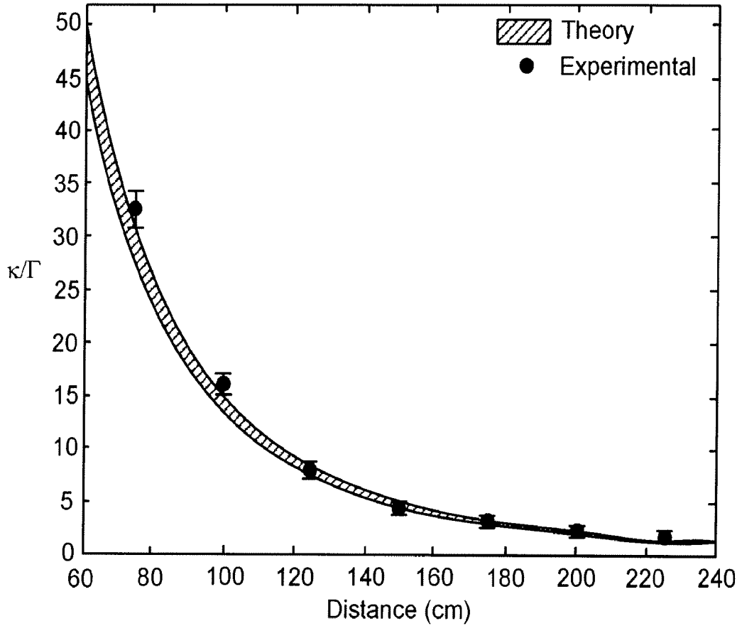
Comparison of experimental and theoretical values for the parameter \kappa/\Gamma as a function of the separation between the two coils. The theory values are obtained by using the theoretically obtained \kappa and the experimentally measured \Gamma . The shaded area represents the spread in the theoretical \kappa/\Gamma due to the ~5% uncertainty in Q .
