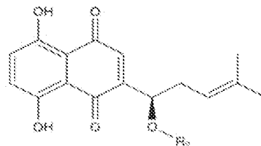
Acetylshikonin derivatives
