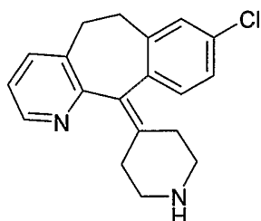
Chemical Structure
