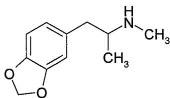
Chemical Structure
