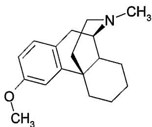
Chemical Structure
