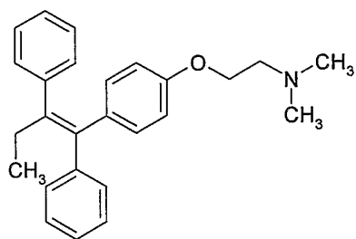
Chemical Structure
