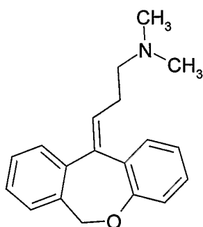
Chemical Structure
