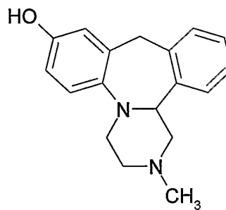
Hydroxylated Metabolite
