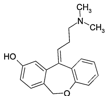
Hydroxylated Metabolite
