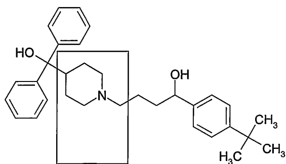
Terfenadine
