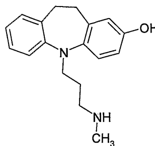
Hydroxylated Metabolite
