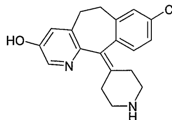
Hydroxylated Metabolite
