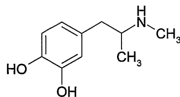
Hydroxylated Metabolite
