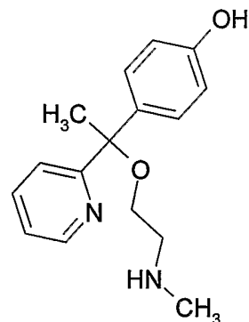
Hydroxylated Metabolite
