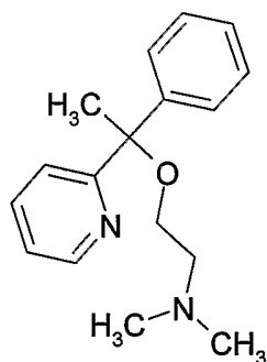
Chemical Structure
