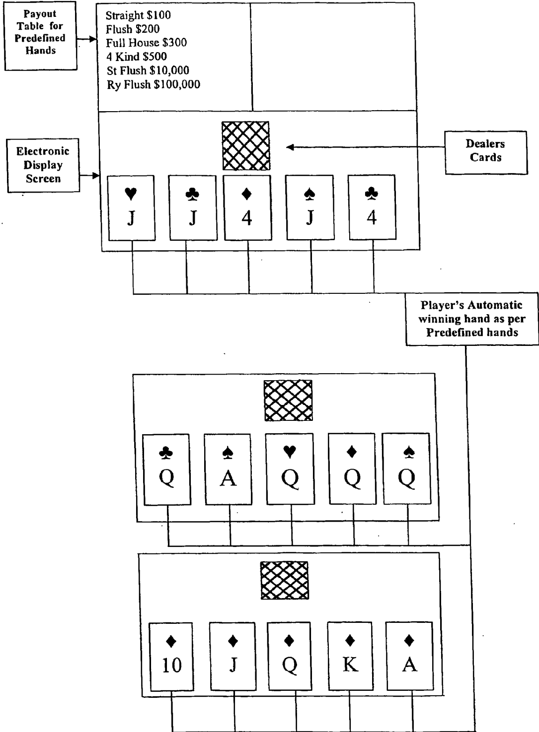
FIGURE 3 PREDEFINED HANDS
