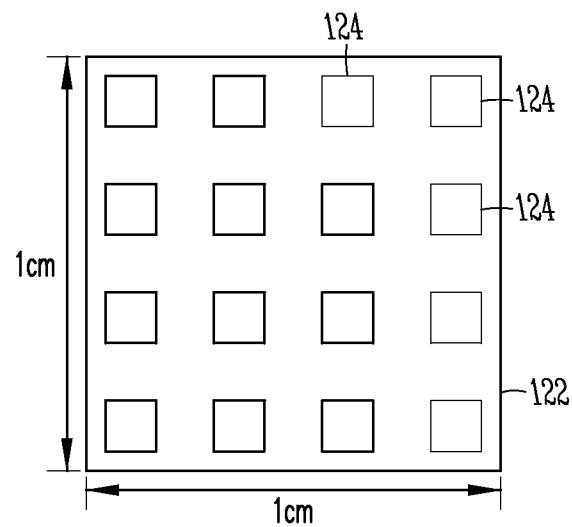
PORTION OF AN ANTENNA ARRAY
