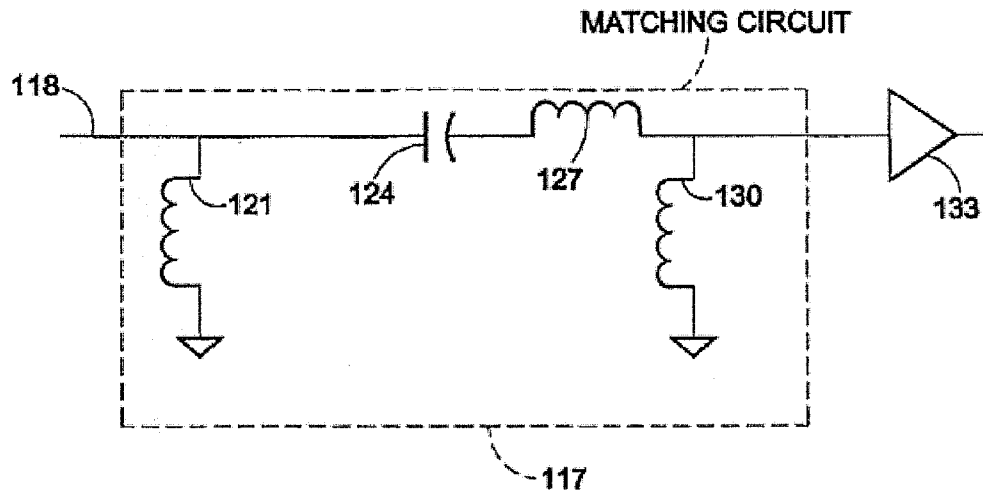
FIG. 6A LNA MATCHING CIRCUIT
