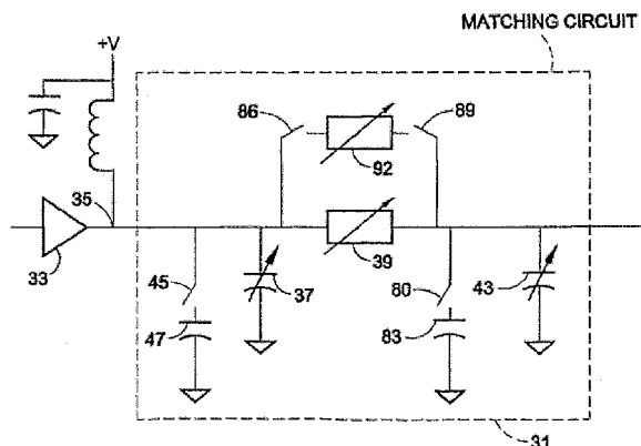
MULTIBAND POWER AMPLIFIER MATCHING CIRCUIT
