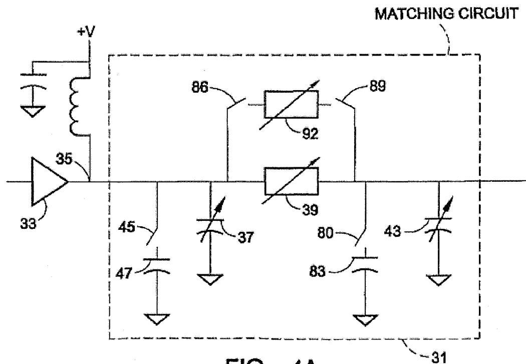
FIG. 4A MULTIBAND POWER AMPLIFIER MATCHING CIRCUIT
