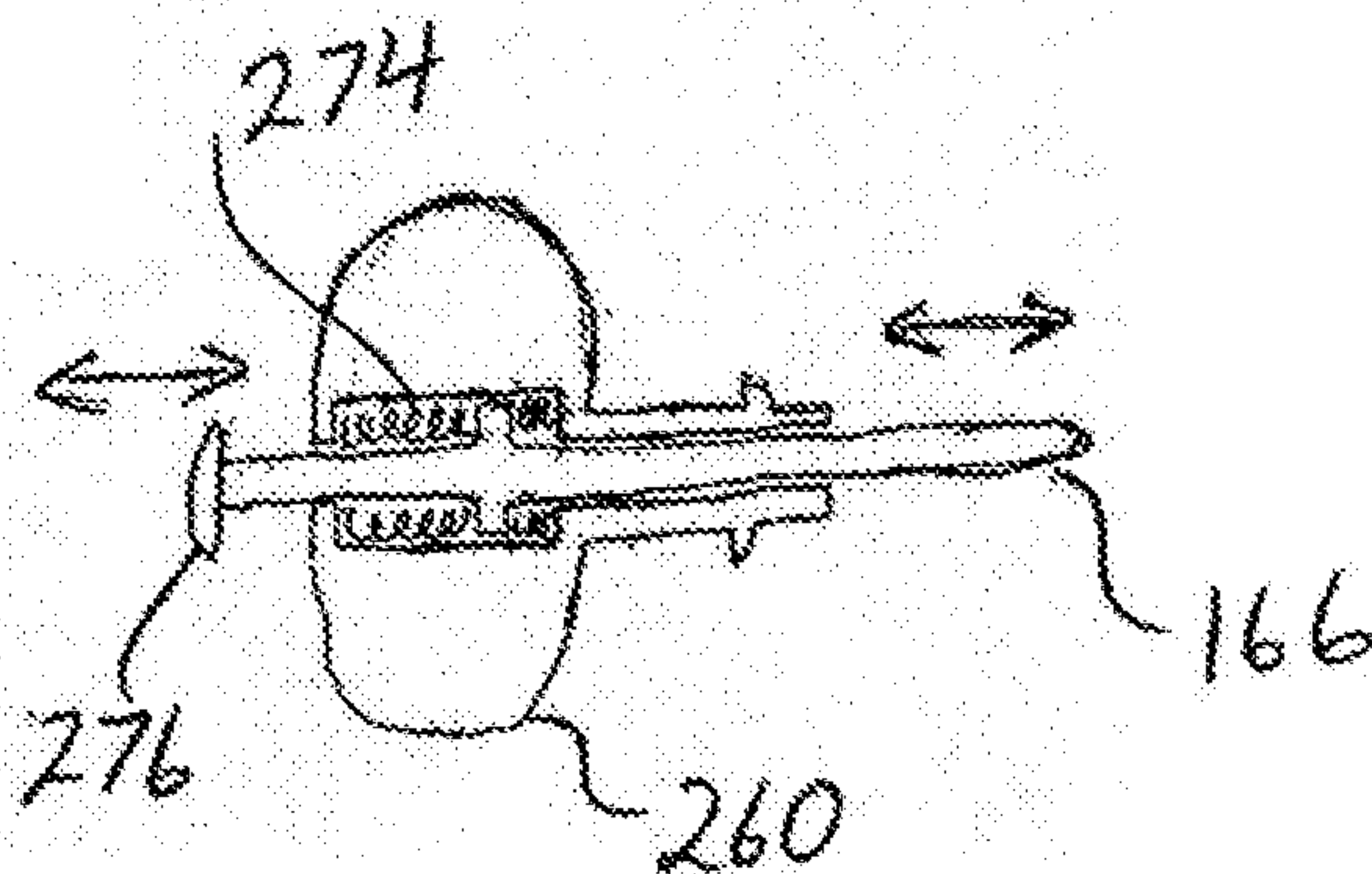
FIG. 107. Extendable and retractable (i.e. for safety) extensions
