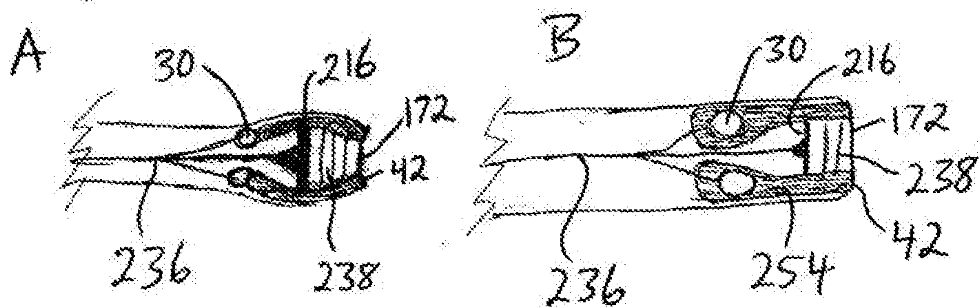
FIG. 96. Lighting and tip configurations – side view (x-sect)
