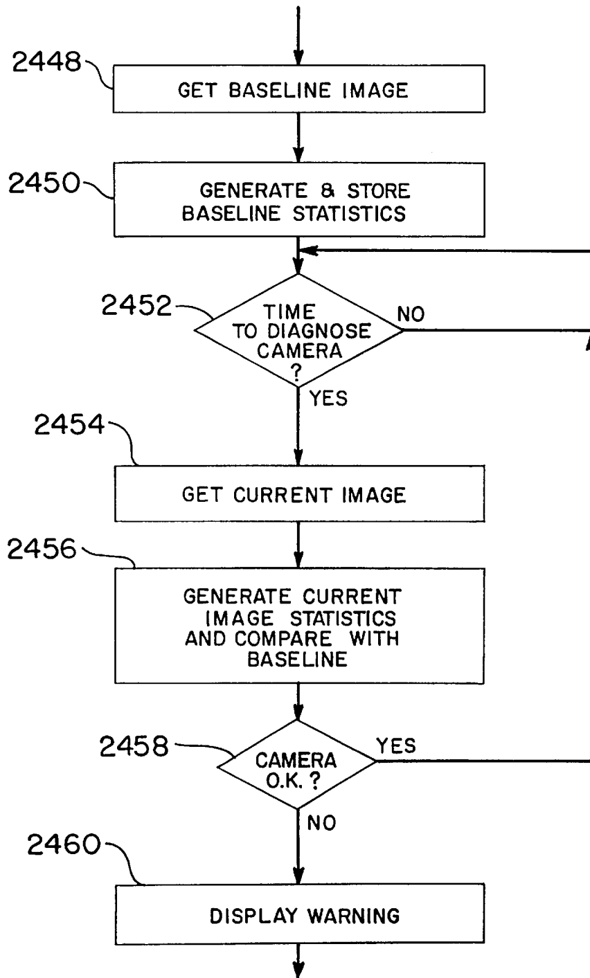
FIG. 120 CAMERA AUTO-DIAGNOSIS
