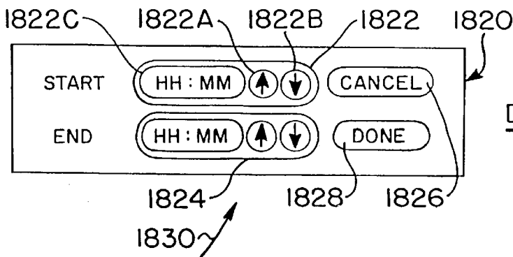
FIG. 85 SCHEDULE QUEUE
