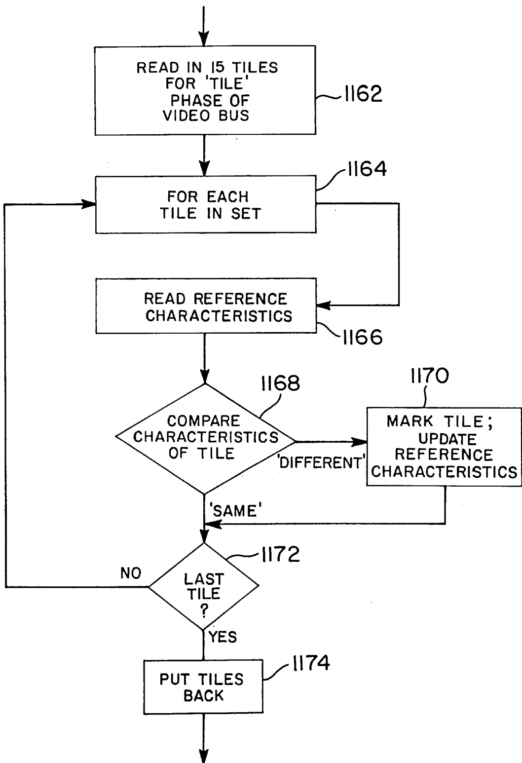
FIG. 42 TILE COMPARING
