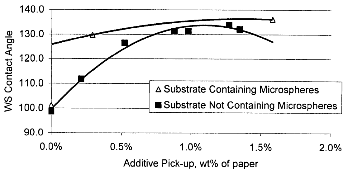
Fig. 4. Wire Side Contact Angle
