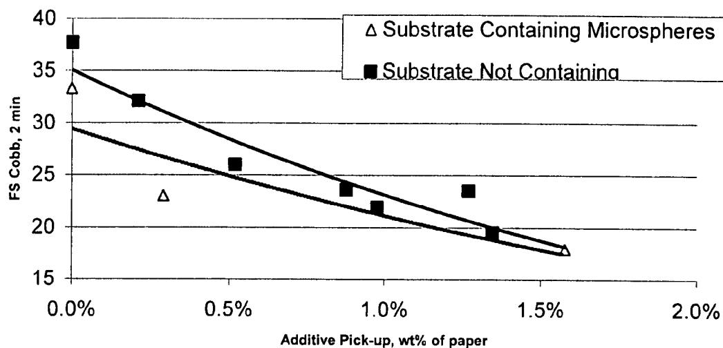
Fig. 1. Felt Side Cobb Size Test
