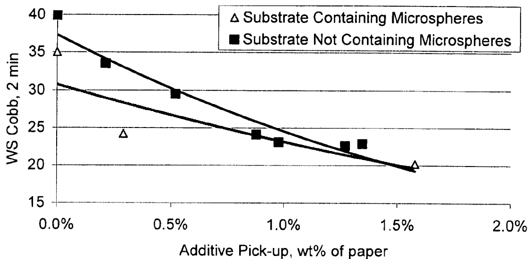
Fig. 2. Wire Side Cobb Size Test
