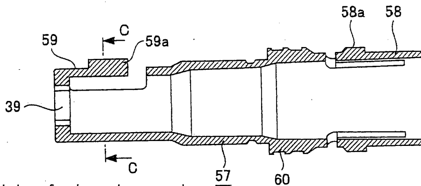
Sectional view of an inner sleeve member
