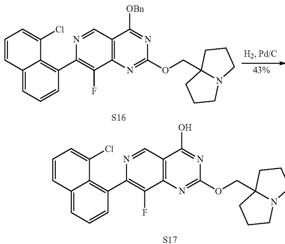
7-(8-chloro-1-naphthyl)-8-fluoro-2-(1,2,3,5,6,7-hexahydropyrrolizin-8-ylmethoxy)pyrido[4,3-d]pyrimidin-4-ol (S17)
