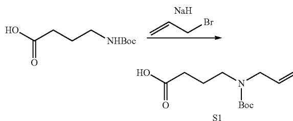
4-(allyl(tert-butoxycarbonyl)amino)butanoic acid (S1)
