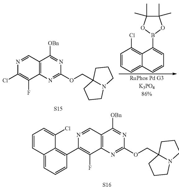
4-benzyloxy-7-(8-chloro-1-naphthyl)-8-fluoro-2-(1,2,3,5,6,7-hexahydropyrrolizin-8-ylmethoxy)pyrido[4,3-d]pyrimidine (S15)
