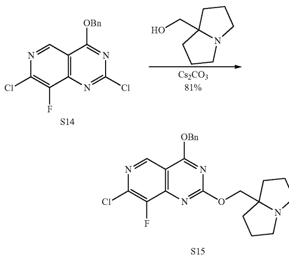
4-(benzyloxy)-7-chloro-8-fluoro-2-((tetrahydro-1H- pyrrolizin-7a(5H)-yl)methoxy)pyrido[4,3-d]pyrimi- dine (S15)
