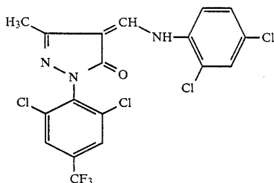
(Variation [(Ia)-β])
