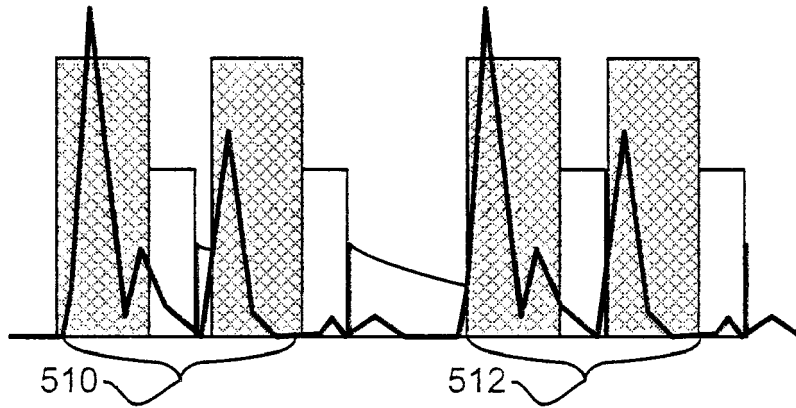
Overdetecting T-Waves
