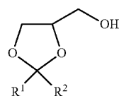
2,2-Dialkyl-4-hydroxymethyl-1,3-dioxolane (Dioxolane)
