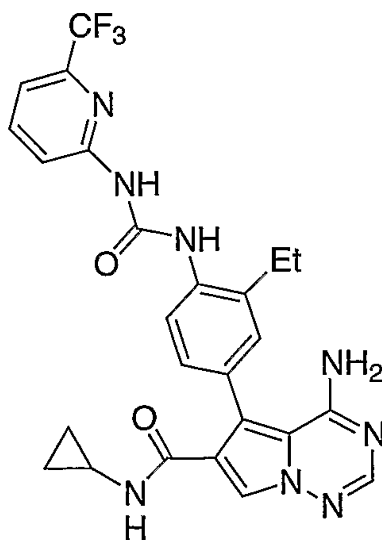
4-amino-N-cyclopropyl-5-{3-ethyl-4-[[[6-(trifluoromethyl)pyridin-2-yl]amino]carbonyl]amino]phenyl}pyrrolo[2,1-f][1,2,4]triazine-6-carboxamide
