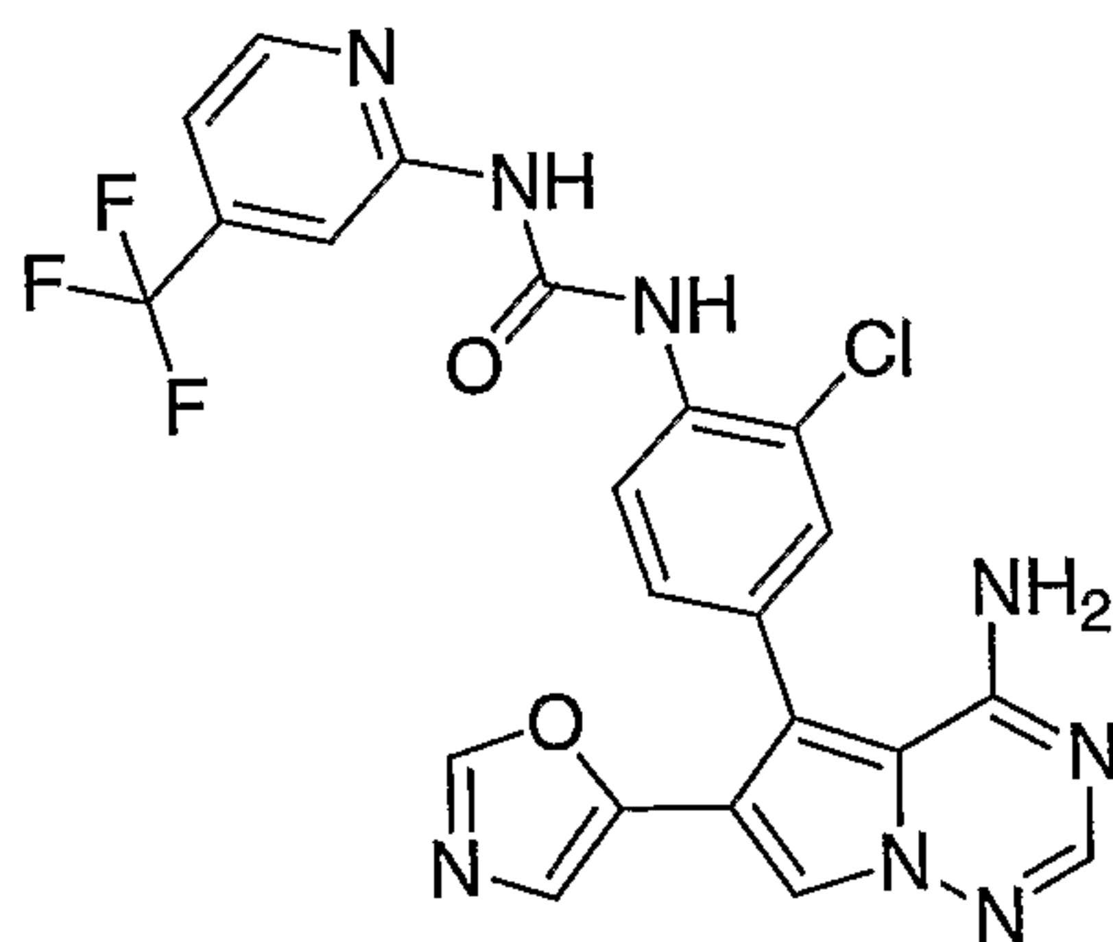
N-{4-[4-amino-6-(1,3-oxazol-5-yl)pyrrolo[2,1-f][1,2,4]triazin-5-yl]-2-chlorophenyl}-N'-[4-(trifluoromethyl)pyridin-2-yl]urea
