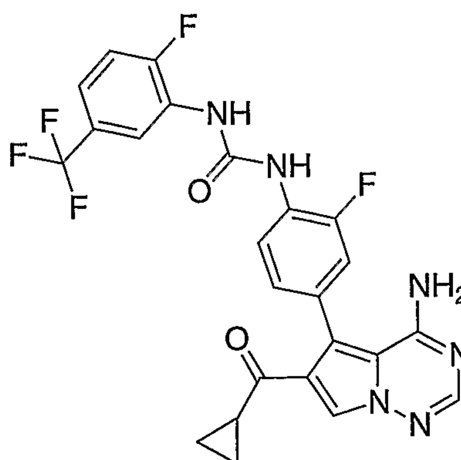
N-[4-(4-amino-6-(cyclopropylcarbonyl)pyrrolo[2,1-f][1,2,4]triazin-5-yl)-2-fluorophenyl]-N'-[2-fluoro-5-(trifluoromethyl)phenyl]urea
