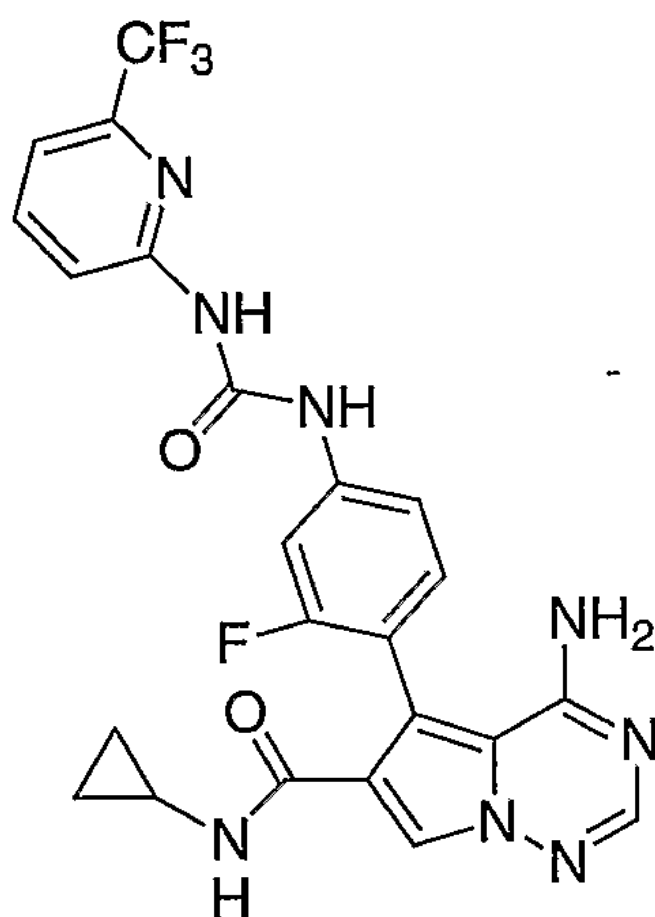
4-amino-N-cyclopropyl-5-{3-ethyl-4-[[[6-(trifluoromethyl)pyridin-2-yl]amino]carbonyl]amino]phenyl}pyrrolo[2,1-f][1,2,4]triazine-6-carboxamide
