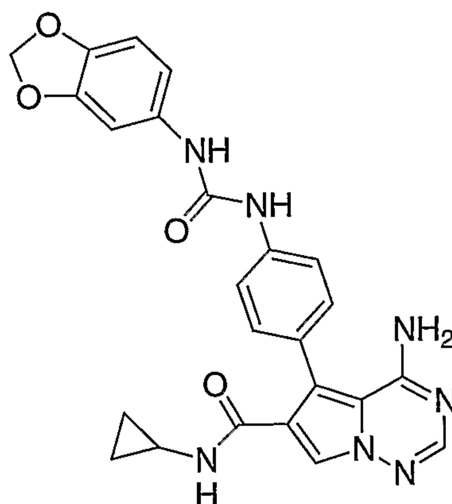
4-amino-5-(4-((1,3-benzodioxol-5-ylamino)carbonyl)amino)phenyl)-N-cyclopropylpyrrolo[2,1-f][1,2,4]triazine-6-carboxamide
