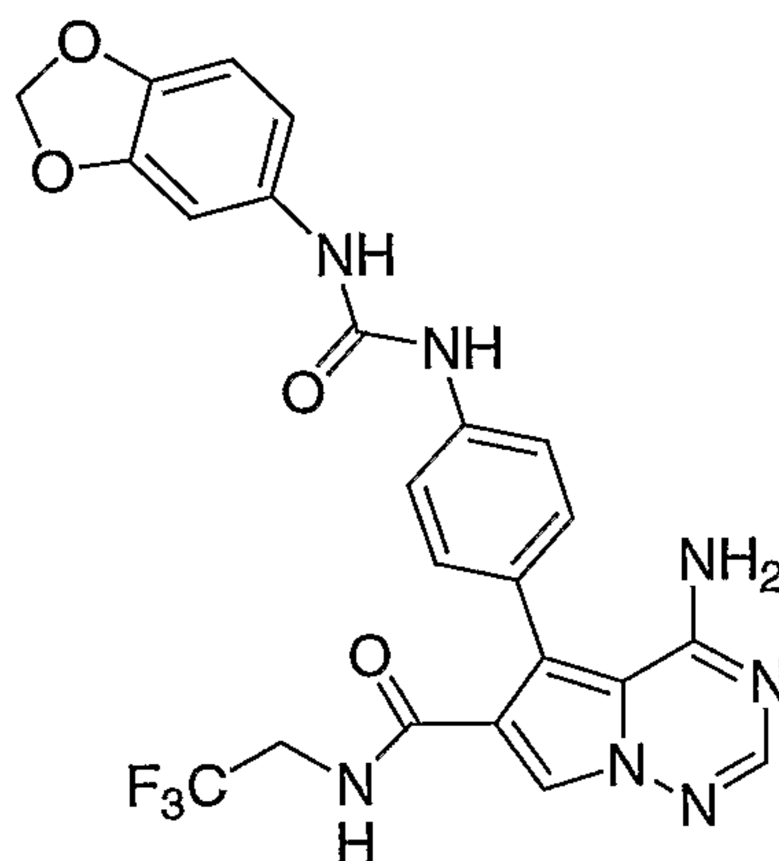
4-amino-5-(4-((1,3-benzodioxol-5-ylamino)carbonyl)amino)phenyl)-N-(2,2,2-trifluoroethyl)pyrrolo[2,1-f][1,2,4]triazine-6-carboxamide
