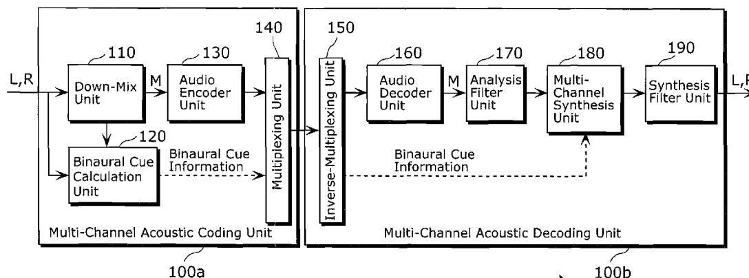
Multi-Channel Acoustic Signal Processing Device 100
