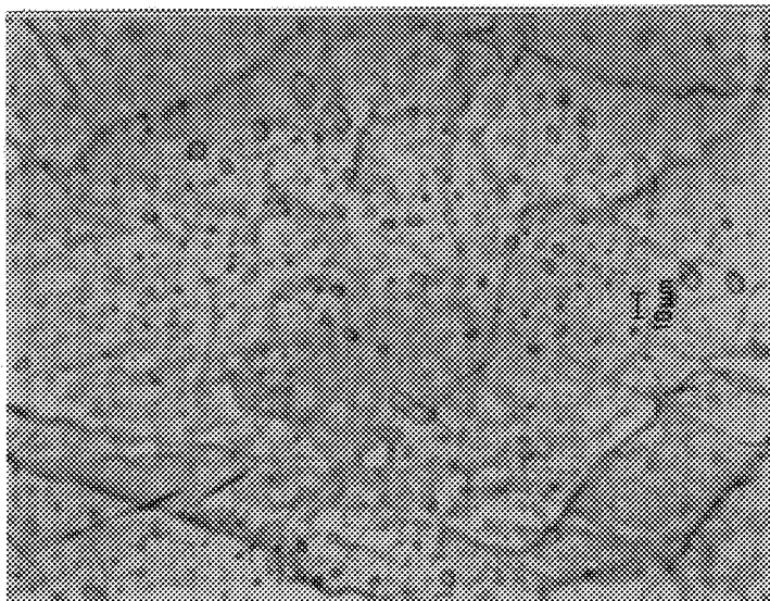
COMP. EX. 1-1(x750) \overline{\hspace{1.5cm}} 20µm
