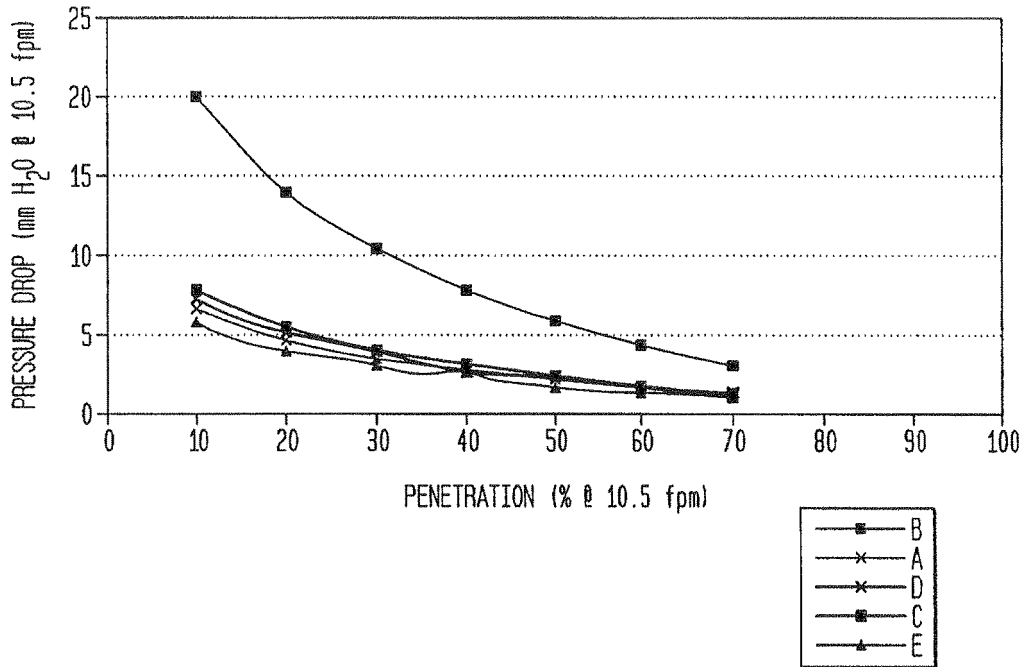
DISCHARGED DOP PENETRATION VERSUS PRESSURE DROP
