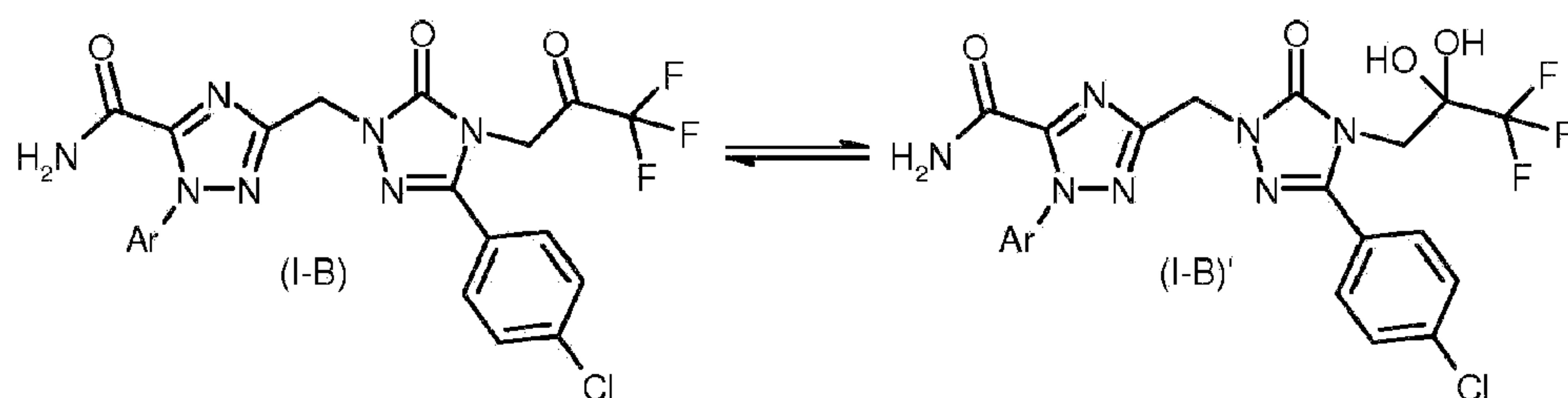
Scheme 1
