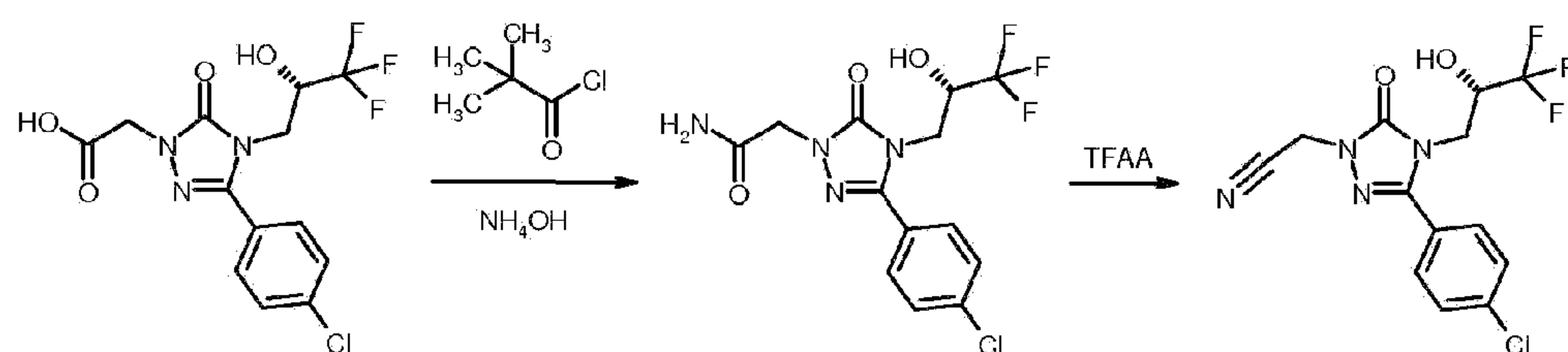
Scheme 6
