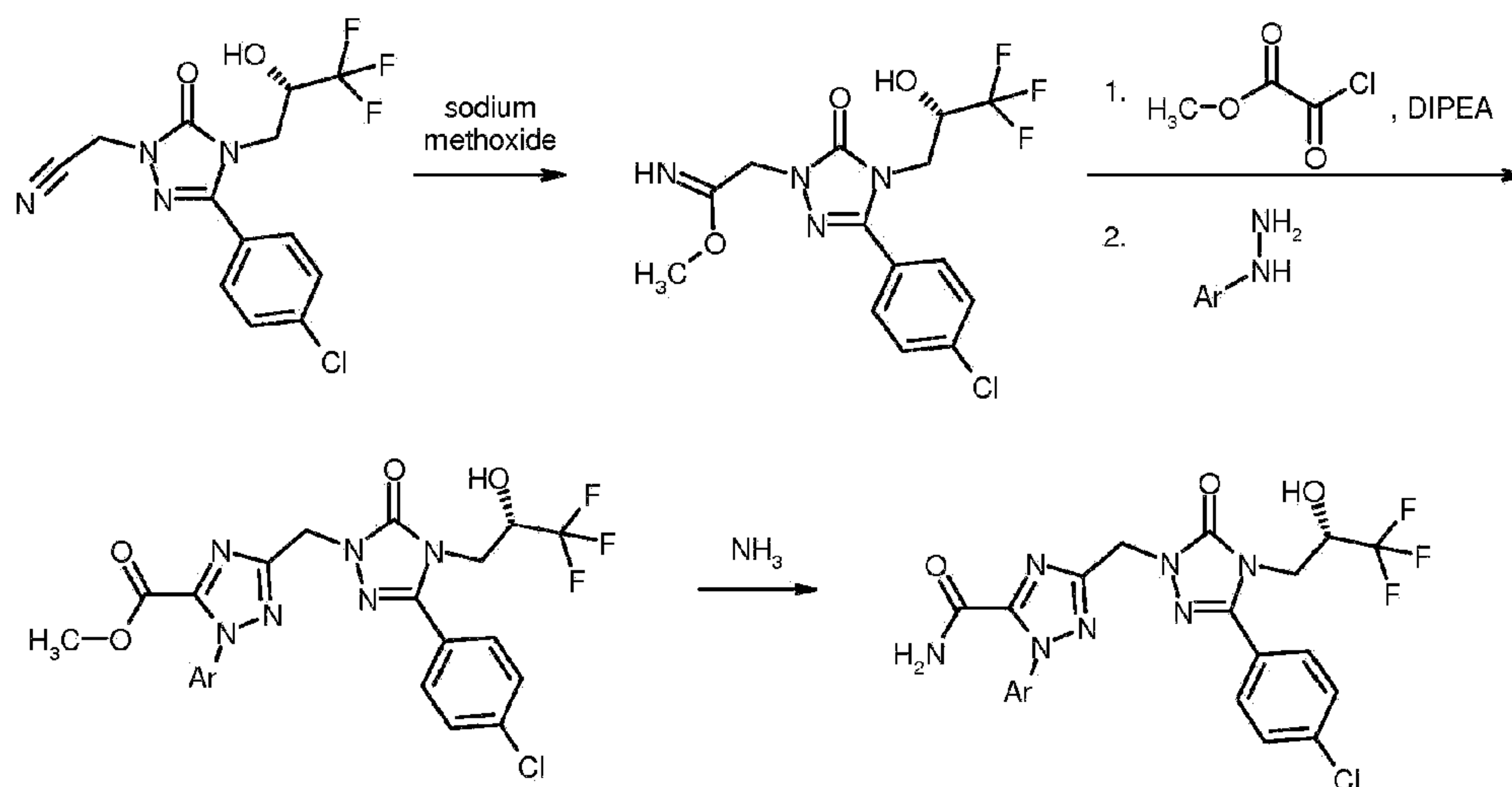
Scheme 7
