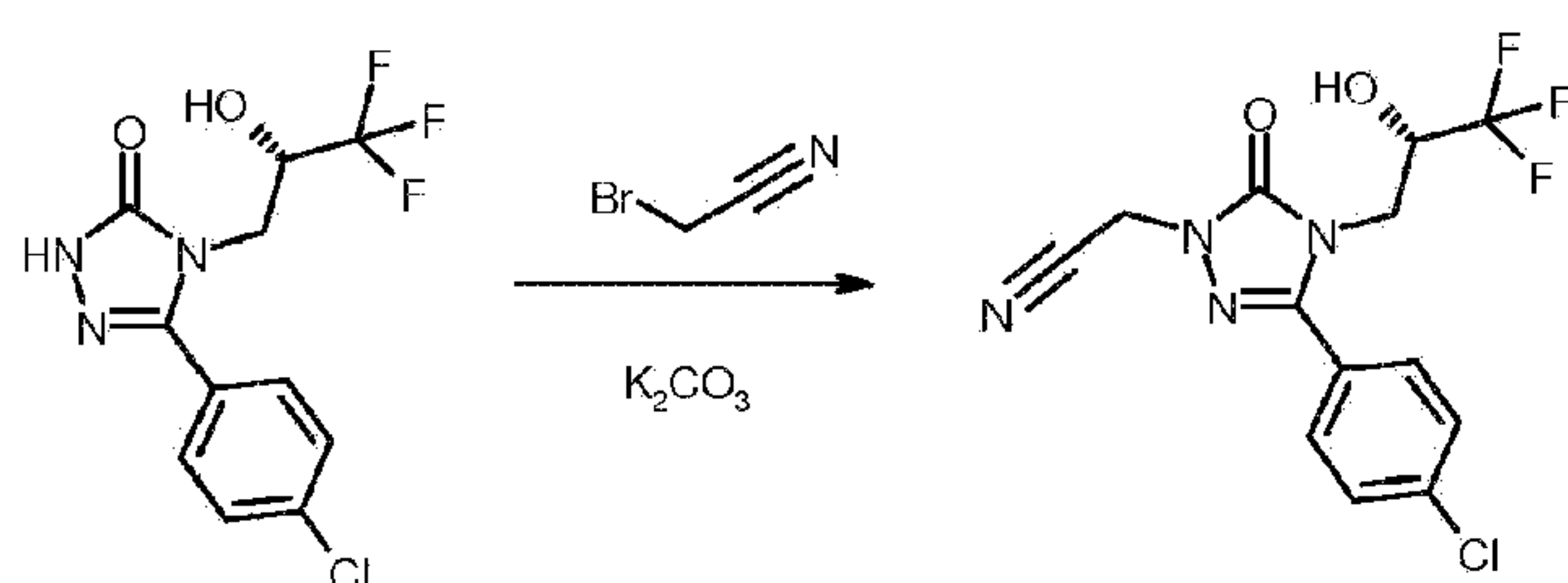
Scheme 7
