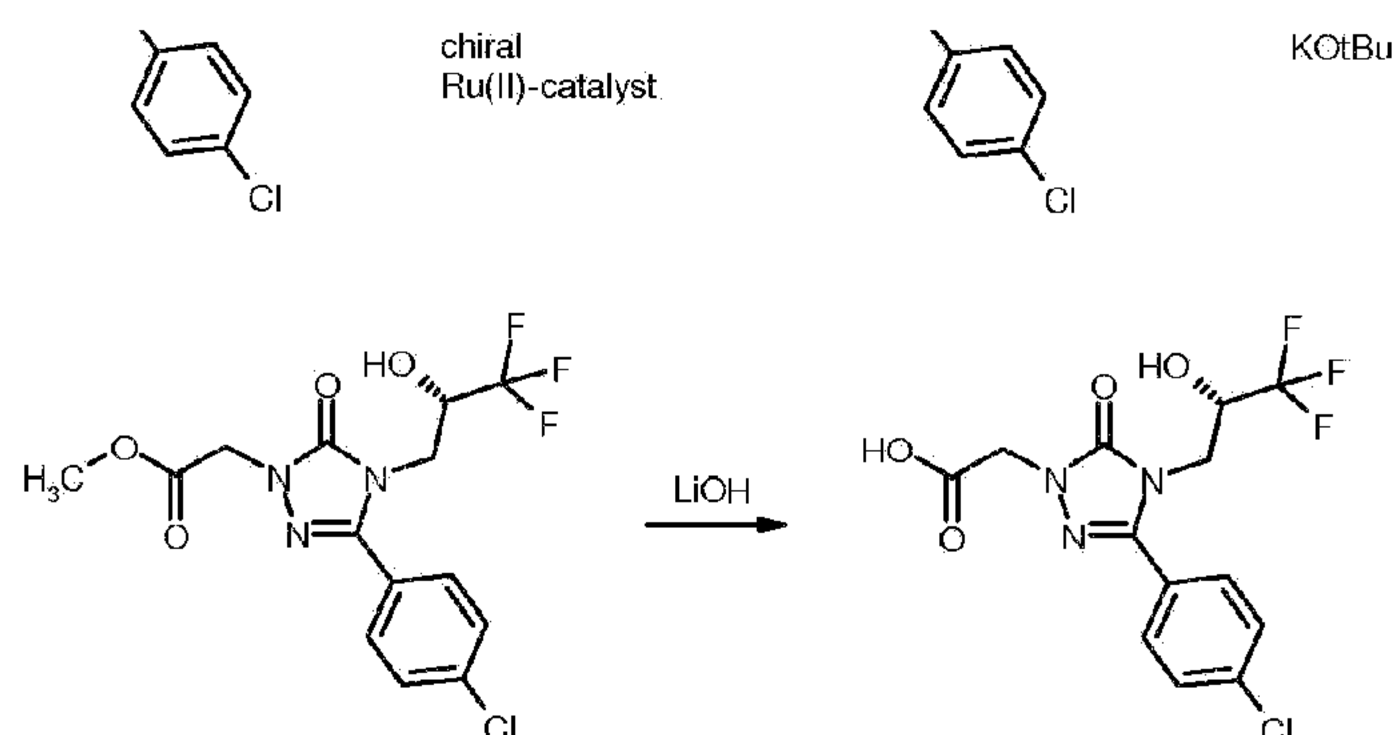
Scheme 5
