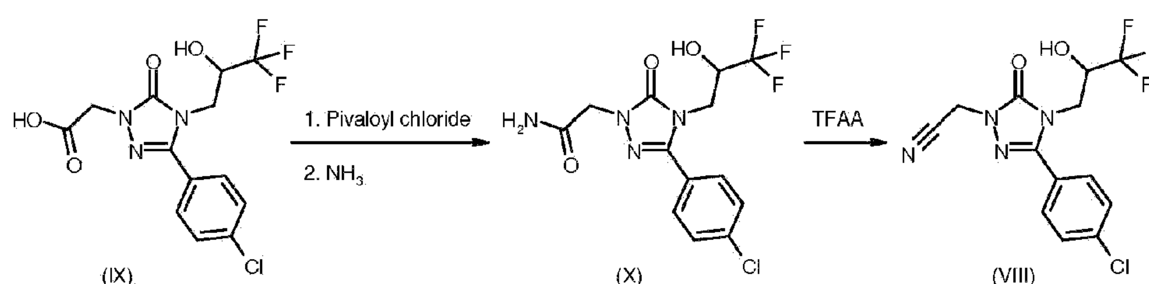
Scheme 2
