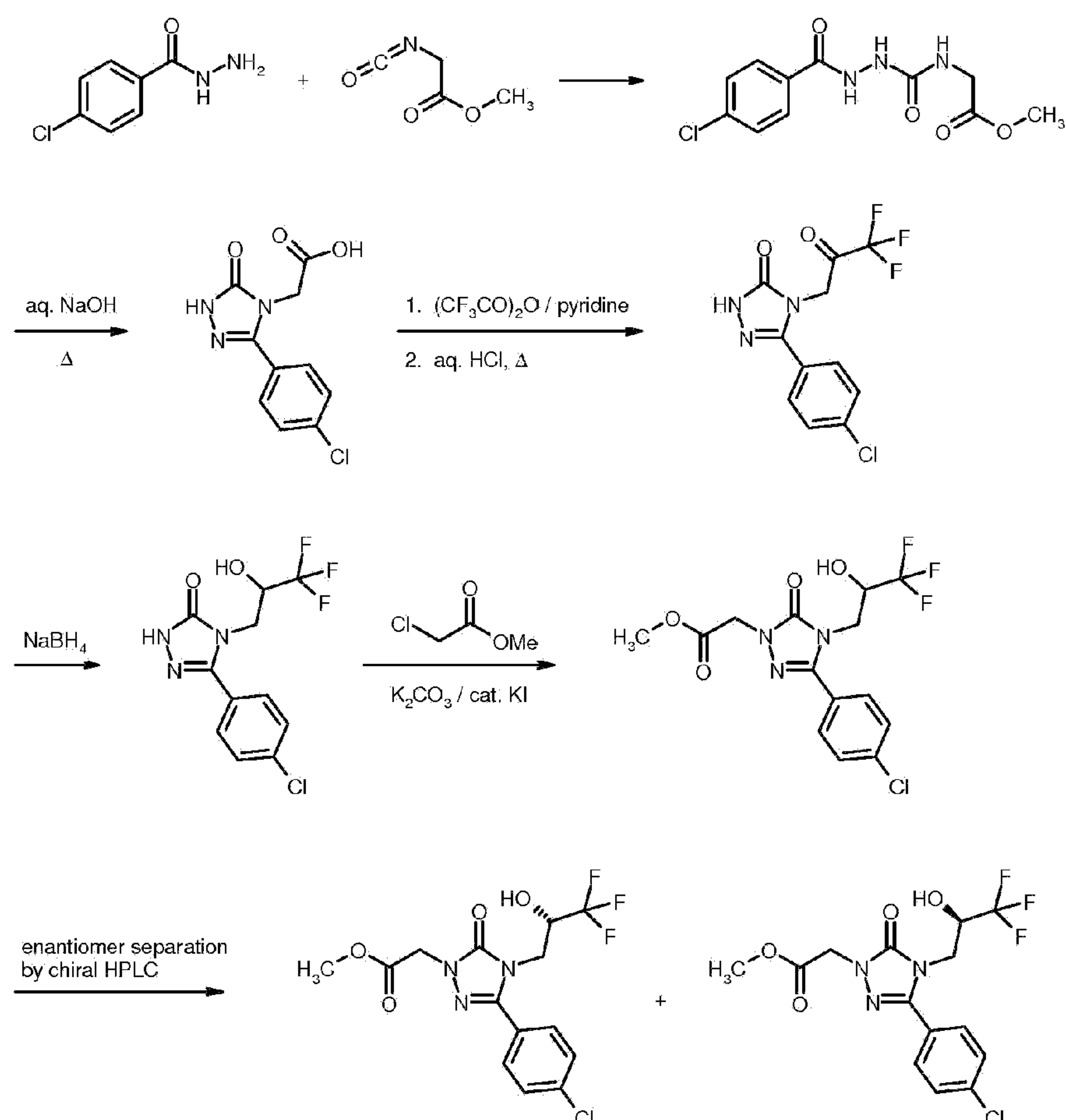
Scheme 4
