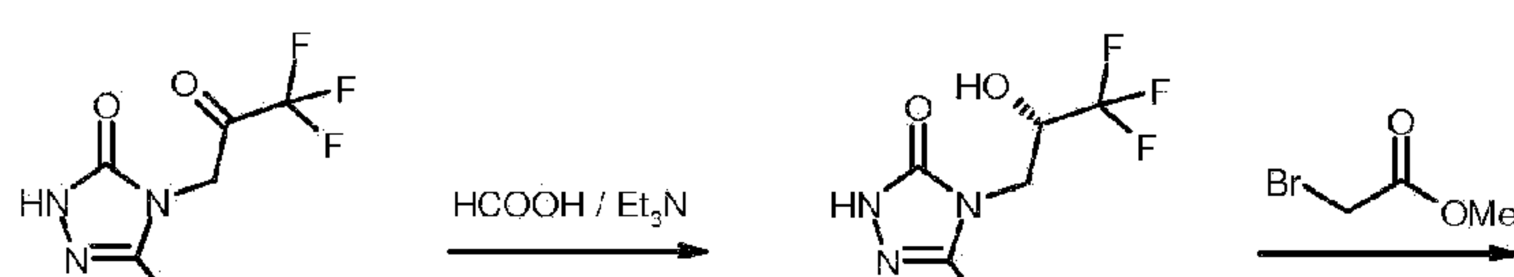
Scheme 4
