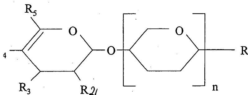
Structure II: Preferred terminal hexose acid group
