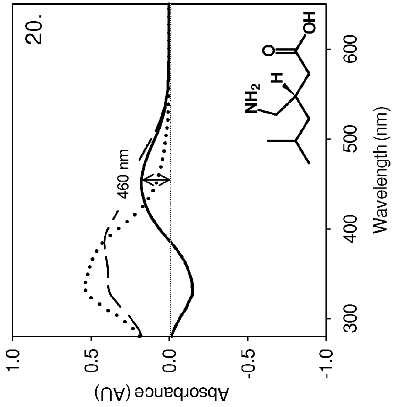
— Differential spectrum between unprotonated and protonated Schiff base.
