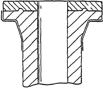
Fig. 1 (PRIOR ART)
