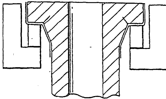
Fig. 3 (PRIOR ART)
