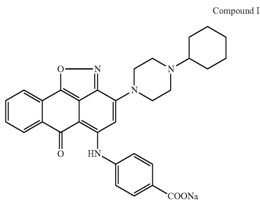
Sodium 4-((3-(4-cyclohexylpiperazin-1-yl)-6-oxo-6H-anthra[1,9-cd]isoxazol-5-yl)amino)benzoate
