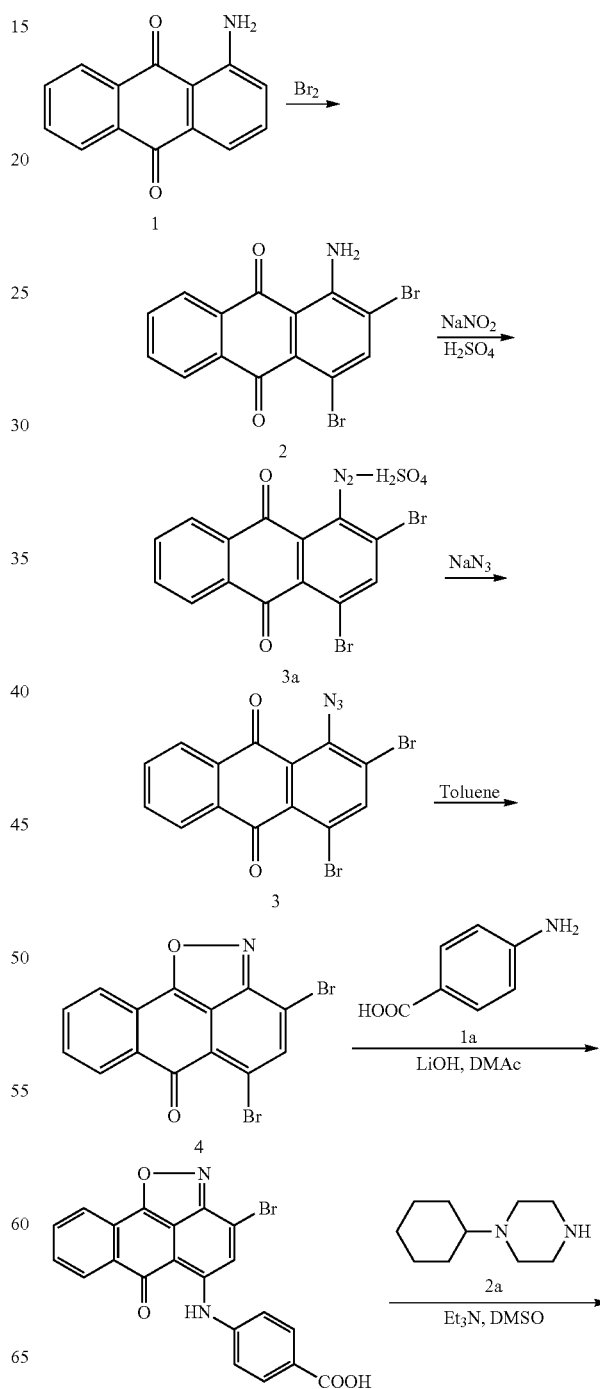
Sodium 4-((3-(4-cyclohexylpiperazin-1-yl)-6-oxo-6H-anthra[1,9-cd]isoxazol-5-yl)amino)benzoate
