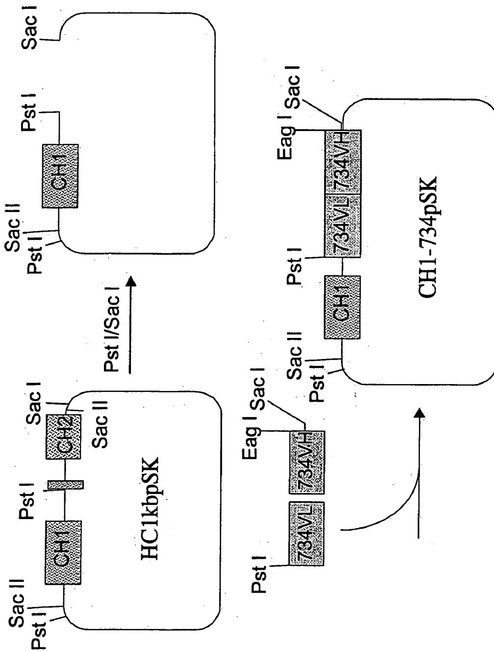
Figure 4. Schematic diagram illustrating production of a 14Fab-734scFv DNA construct.
