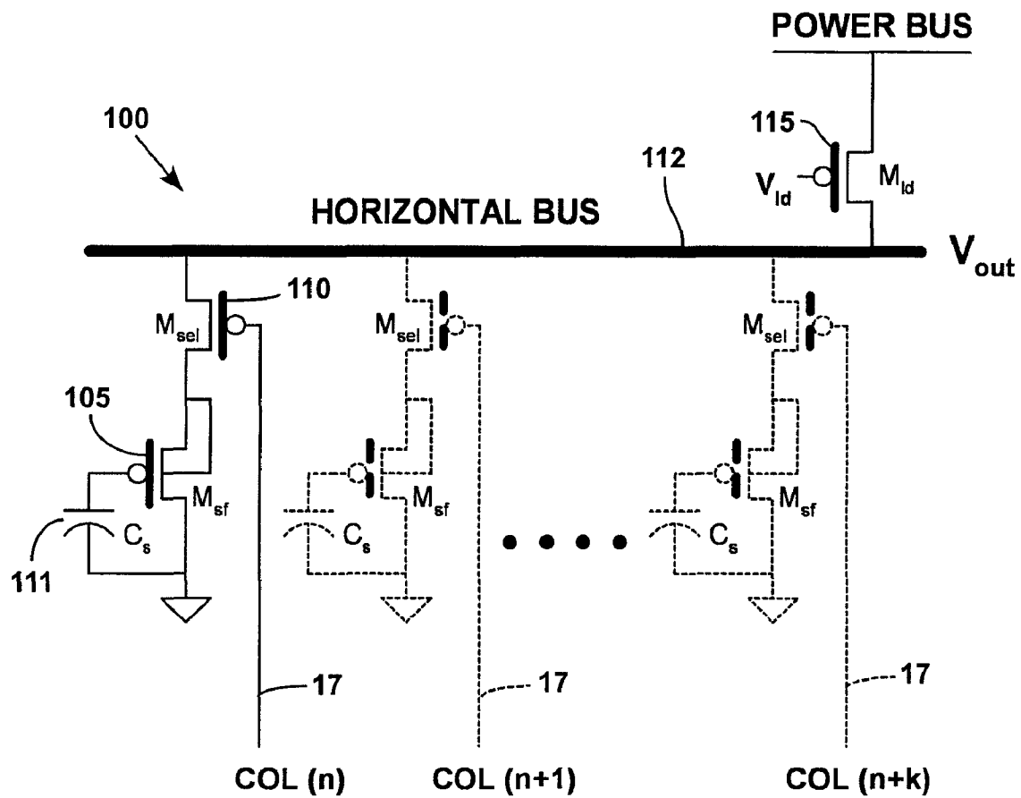
FIG. 4 (PRIOR ART)
