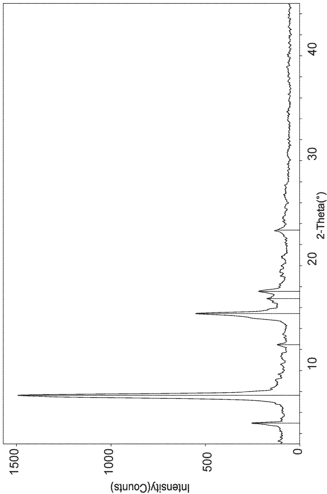
FIG. 22 XRPD: Compound II Ethanesulfonic Acid Salt
