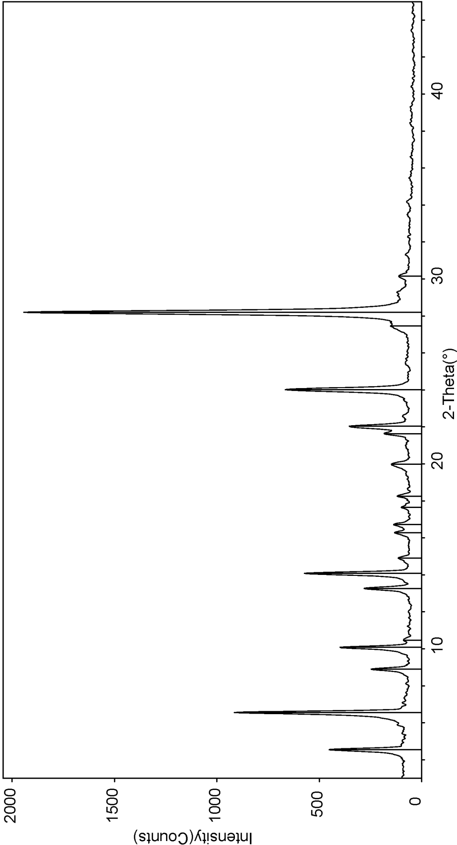
FIG. 7 XRPD: Compound II Maleic Acid Salt
