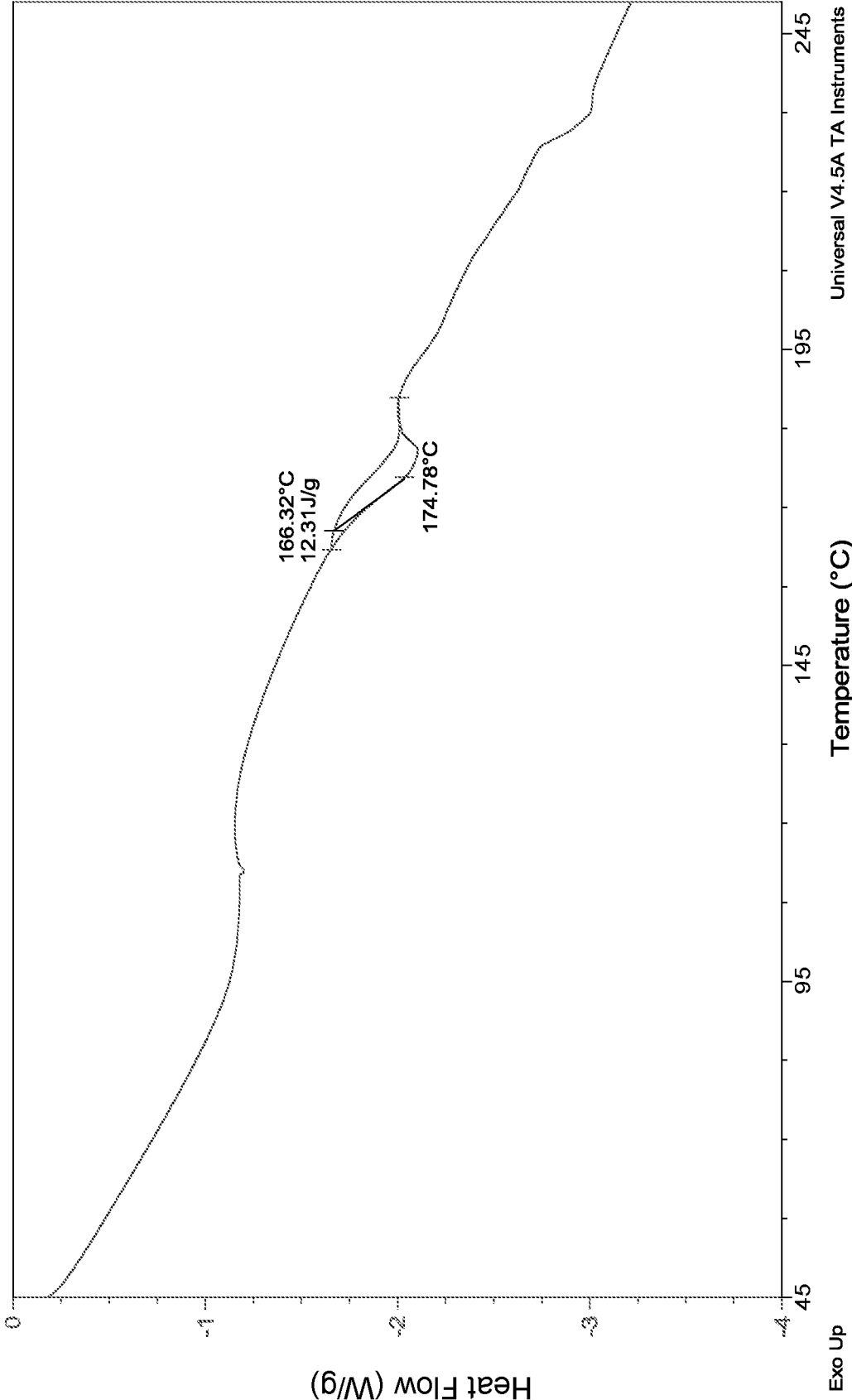
FIG. 20 DSC: Compound II Methanesulfonic Acid Salt
