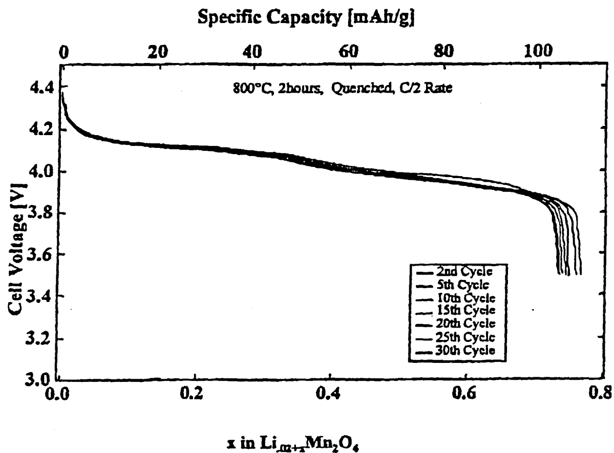
The discharge curves at C/2 rate for a sample of Li-SMD calcined at 800°C for 2 hours and quenched to room temperature.
