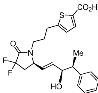
Example 35D
