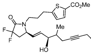
Example 24C
