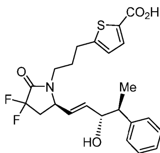
Example 35C
