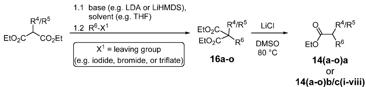
Scheme 7b
