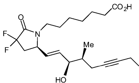
Example 2D
