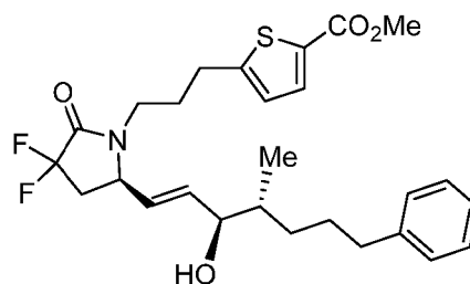
Example 28F
