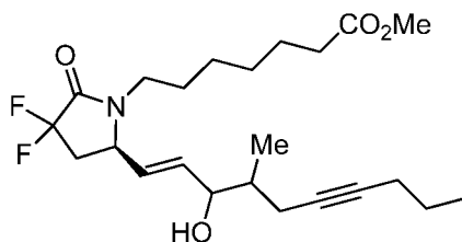
Example 4
