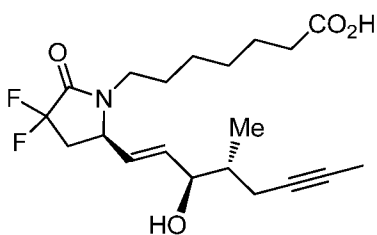
Example 1I
