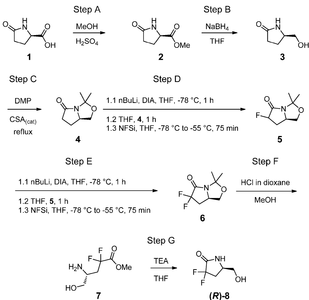
Scheme 1
