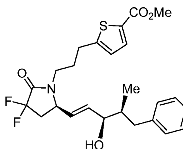
Example 36B
