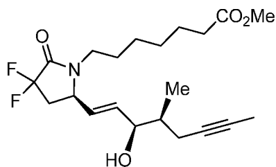
Example 1D
