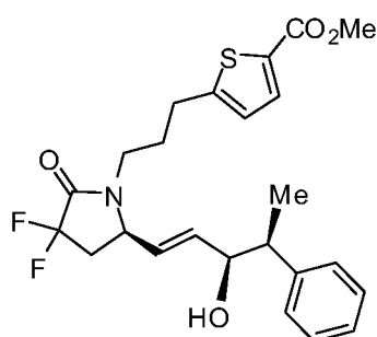
Example 35B
