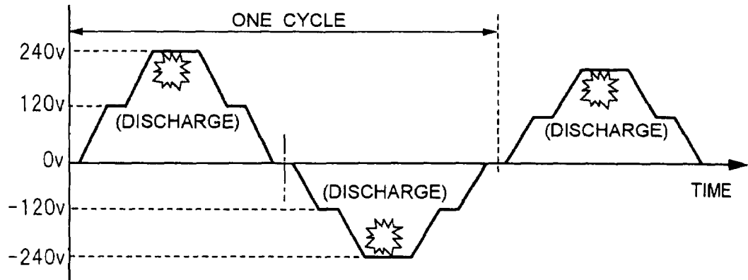
FIG. 7C VOLTAGE WAVEFORM OF (X - Y)
