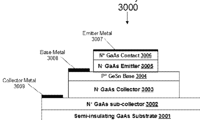
NPN GaAs-GeSn-GaAs symmetric double HBT
