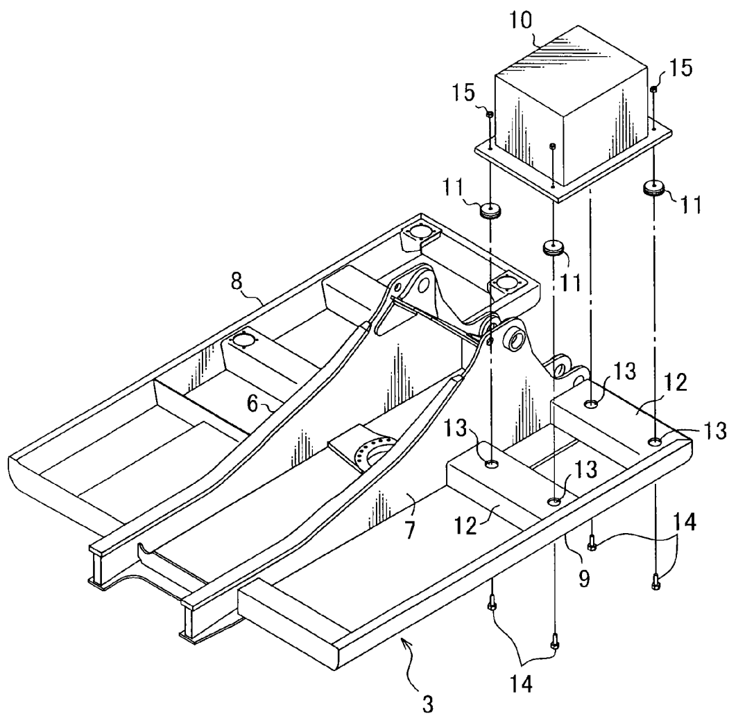
PRIOR ART FIG. 6
