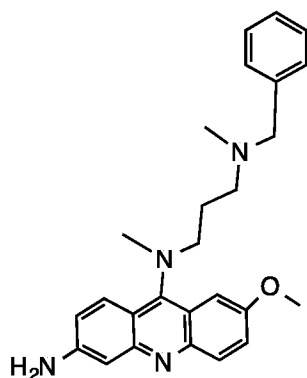
9-(N-benzyl-N-methyl-N'-methyl-1',3'-propanediamine)-3-amino-7-methoxyacridine (X5)
