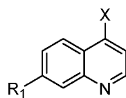
(IIIa)
