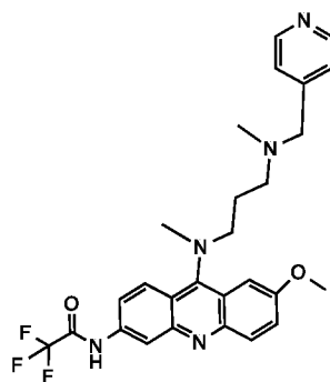
9-(N-(4''-pyridylmethyl)-N-methyl-N'-methyl-1',3'-propanediamine))-3-trifluoroacetamide-7-methoxyacridine (TFA X6)
