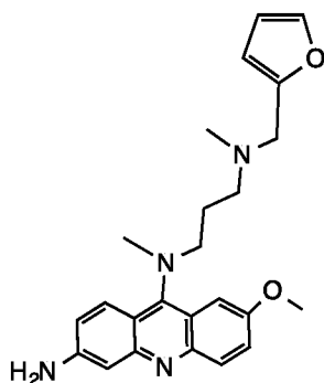
9-(N-furfuryl-N-methyl-N'-methyl-1',3'-propanediamine)-3-amino-7-methoxyacridine (X7)
