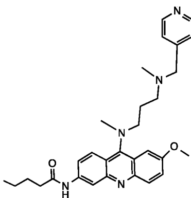
9-(N-(4''-pyridylmethyl)-N-methyl-N'-methyl-1',3'-propanediamine))-3-n-butoxyamino-7-methoxyacridine (C6X6)
