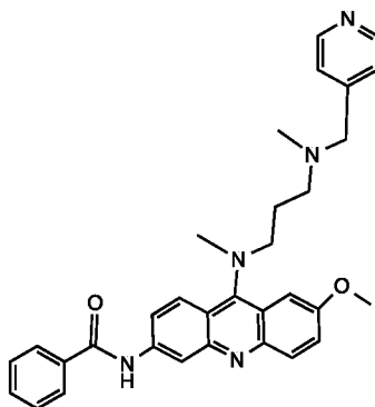
9-(N-(4''-pyridylmethyl)-N-methyl-N'-methyl-1',3'-propanediamine))-3-benzamide-7-methoxyacridine (Bz X6)
