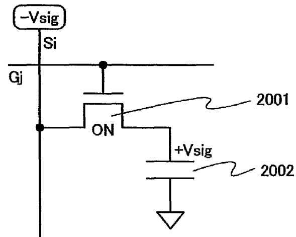
FIG. 20C PRIOR ART
