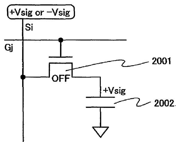
FIG. 20C PRIOR ART
