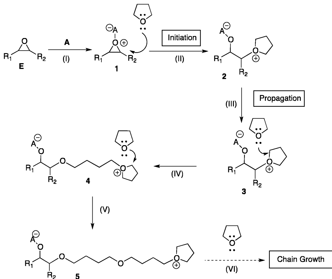
Scheme 1. Hypothesised reaction mechanism for THF polymerisation.
