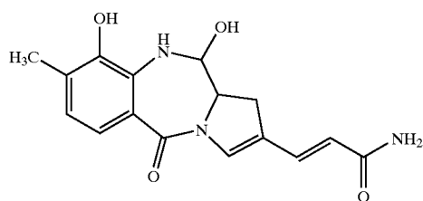
Athramycin
