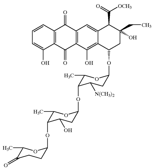
Aciacinomycin A
