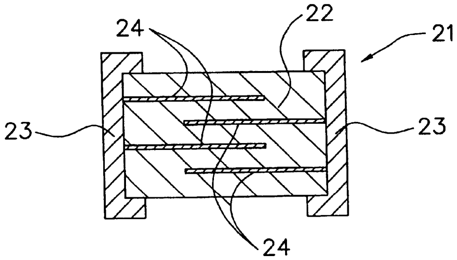
FIG. 3 (PRIOR ART)
