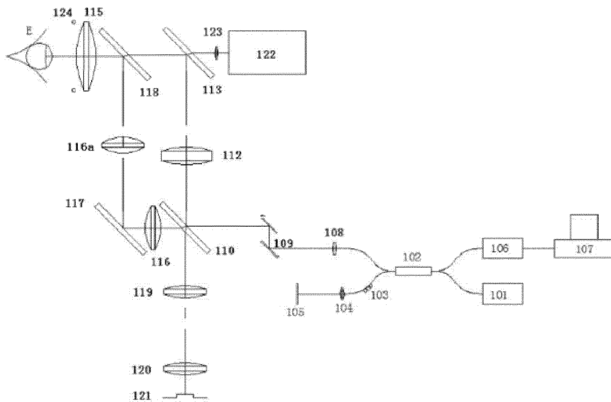
Figure 5 (RELATED ART)
