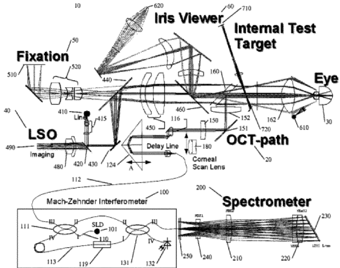
Figure 1 (RELATED ART)
