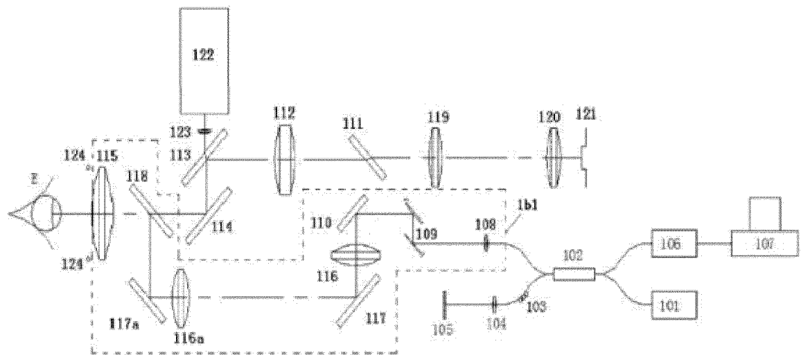
Figure 4 (RELATED ART)
