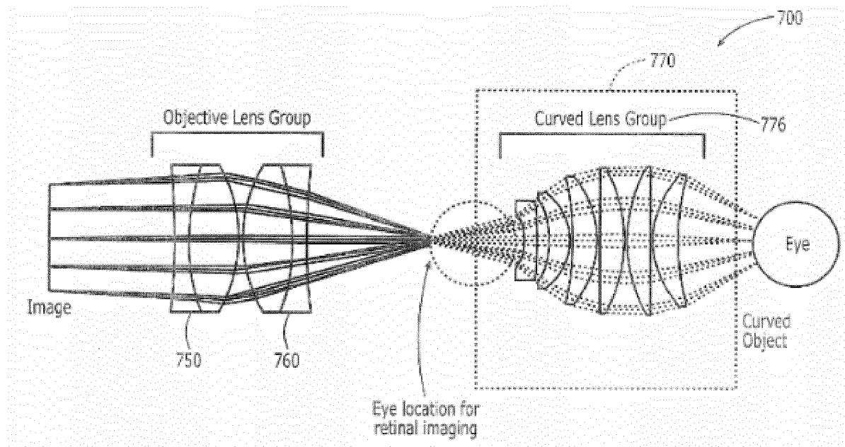
Figure 6 (RELATED ART)
