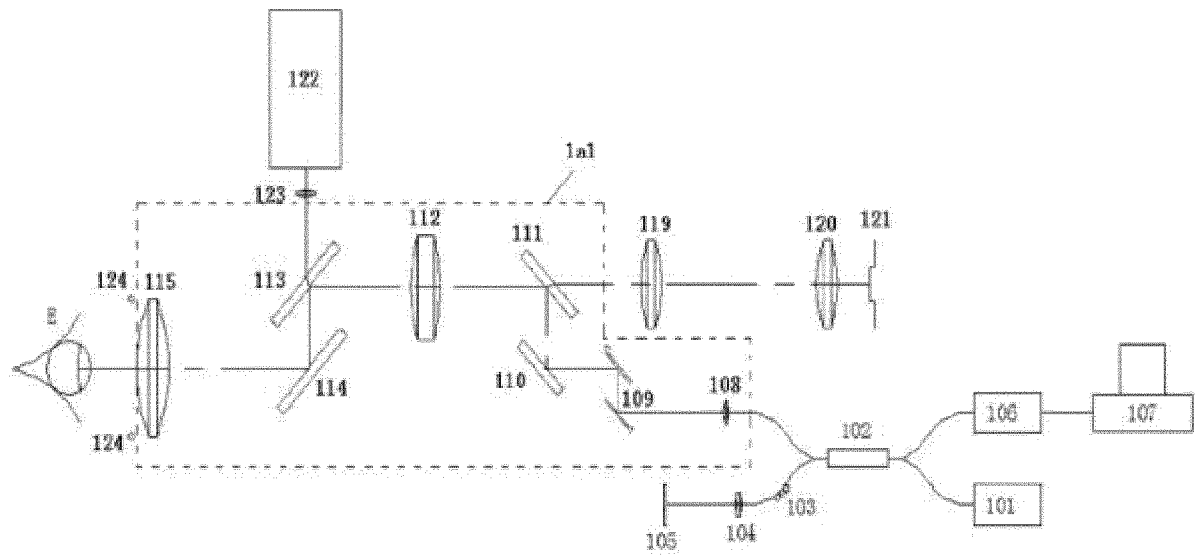
Figure 3 (RELATED ART)
