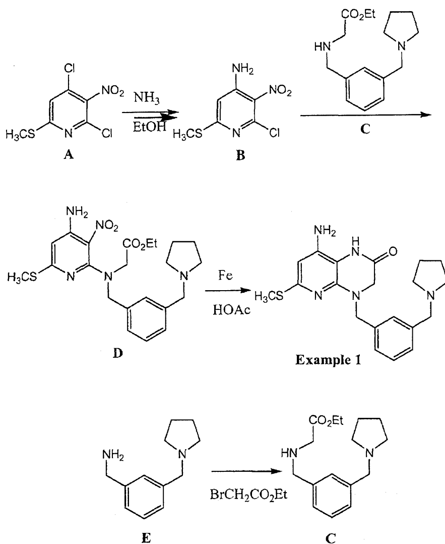
Scheme 1
