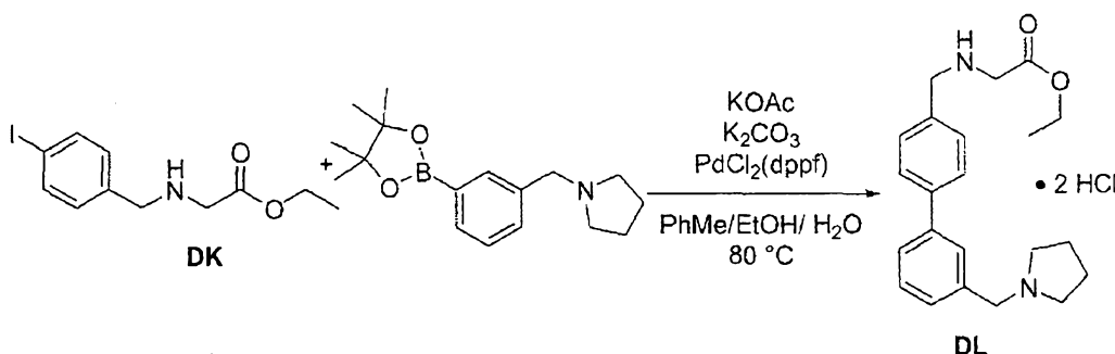
Scheme 78
