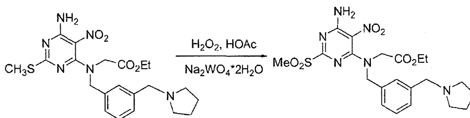
Scheme 11
