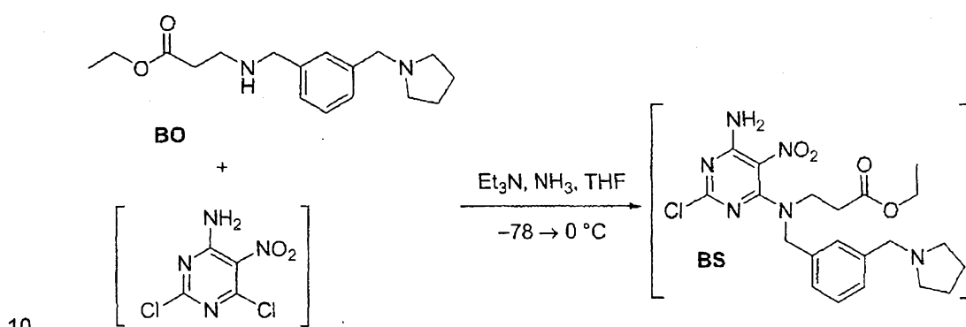
Scheme 40
