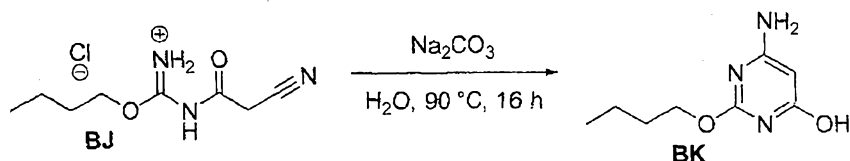
Scheme 29
