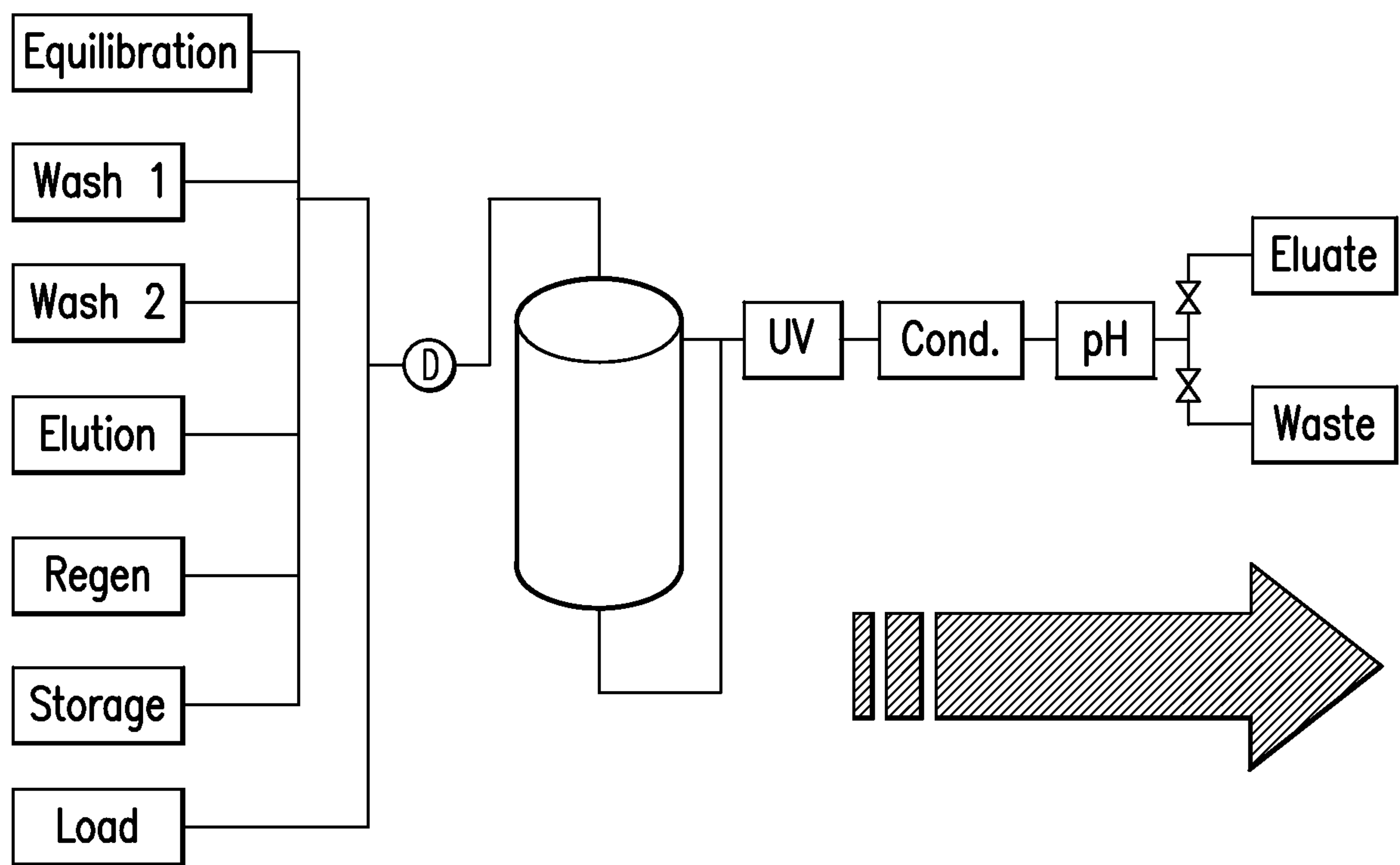
Conventional chromatography flow diagram
