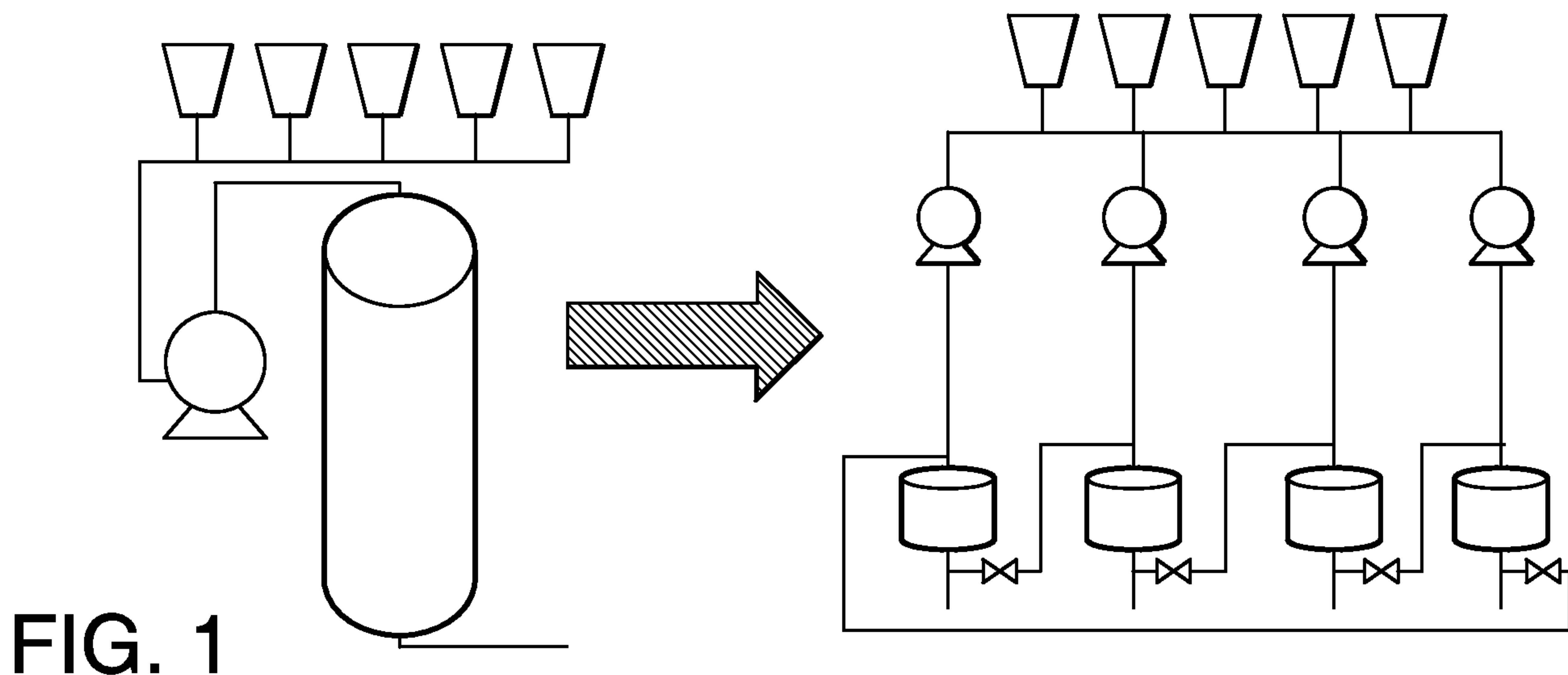
Conventional chromatography flow diagram vs. SMB
