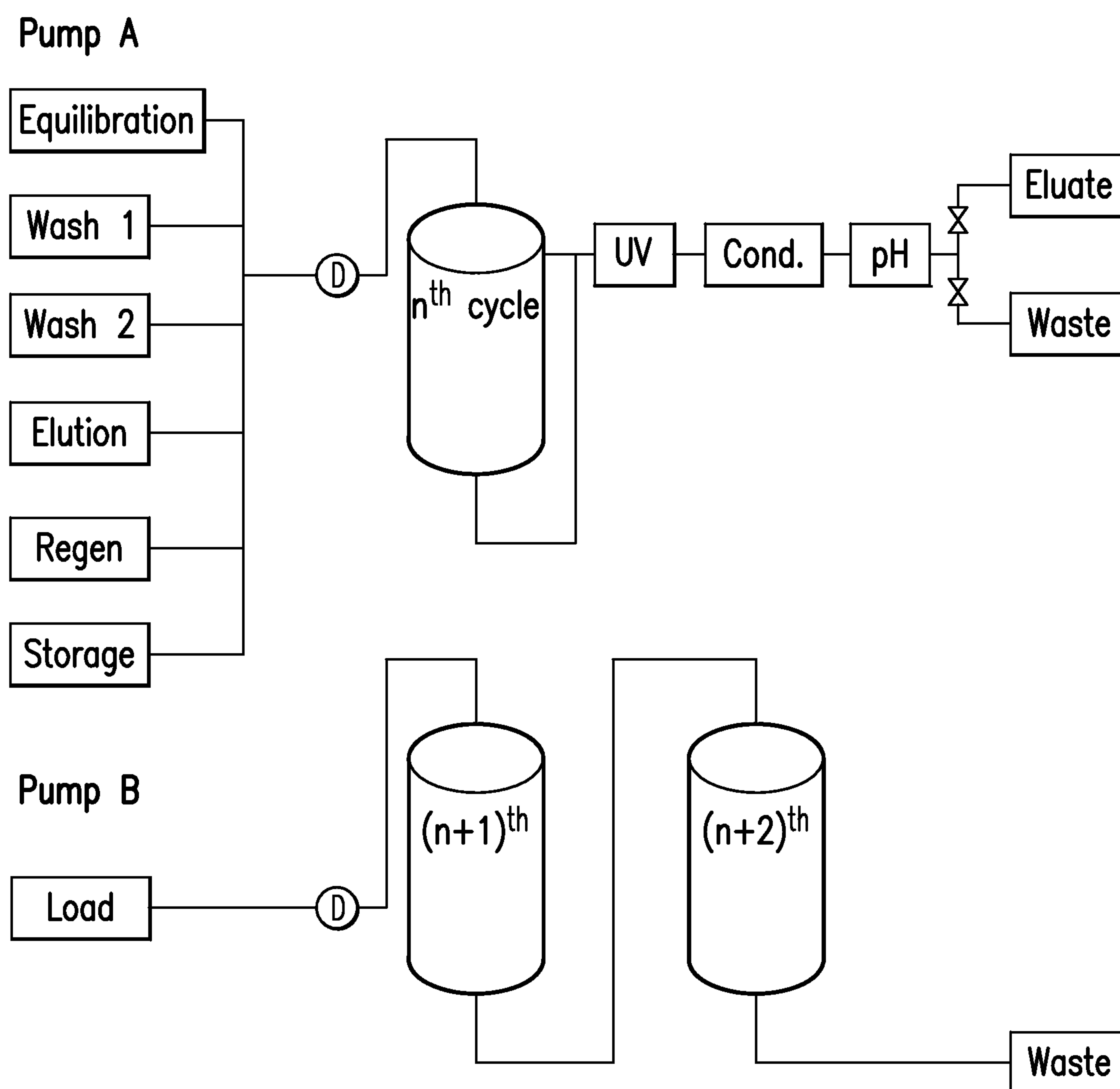
SMB chromatography flow diagram
