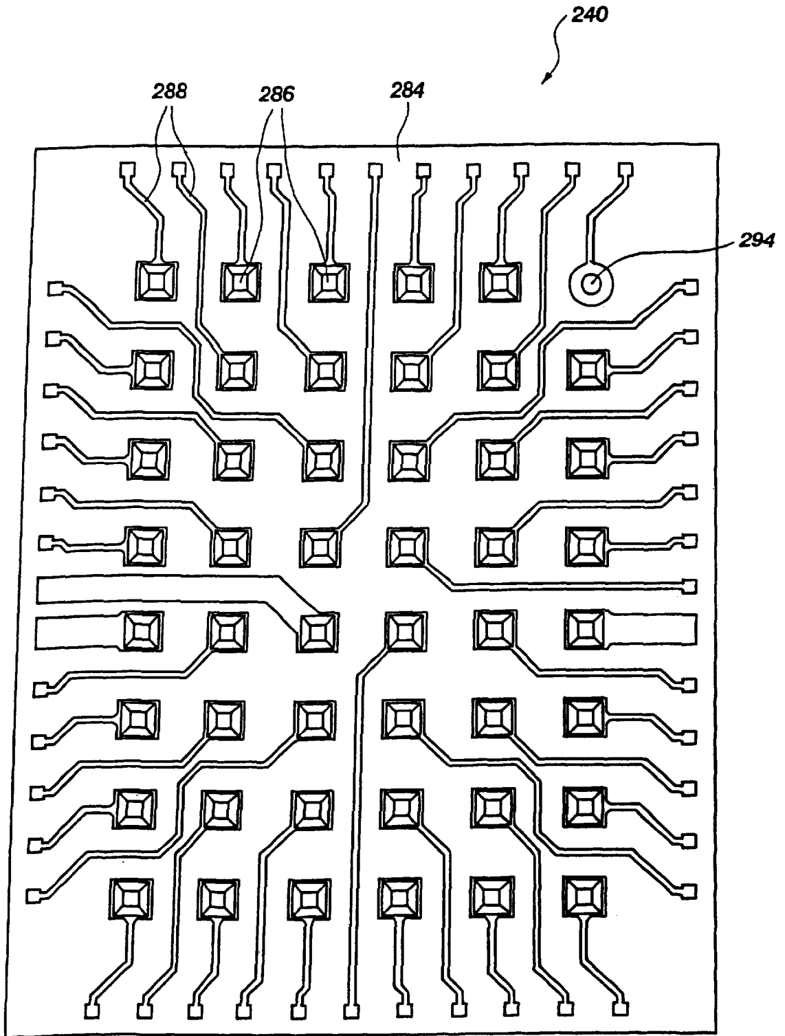
Fig. 12 (PRIOR ART)
