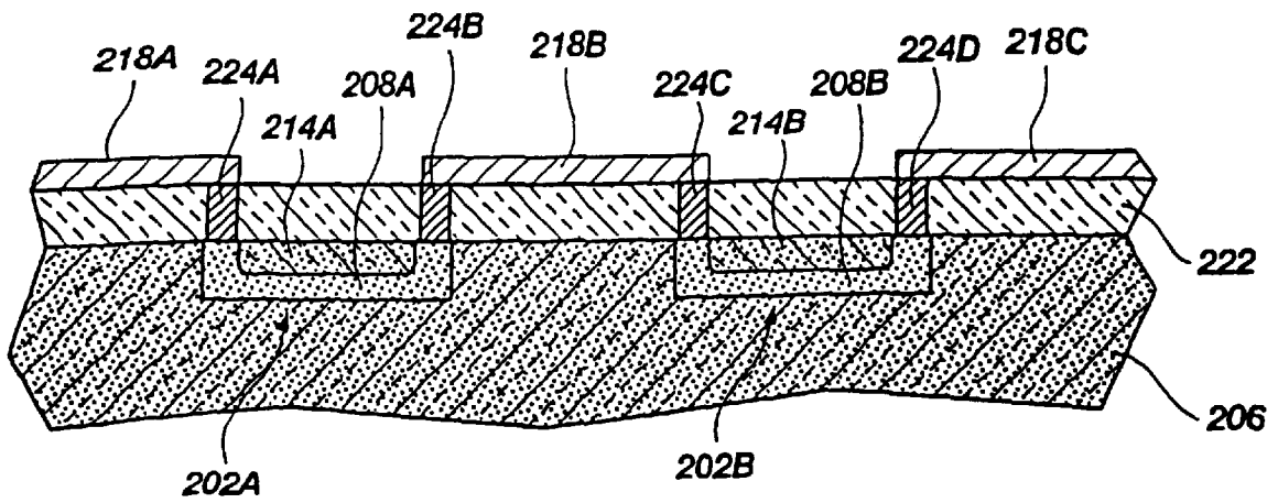
Fig. 10 (PRIOR ART)
