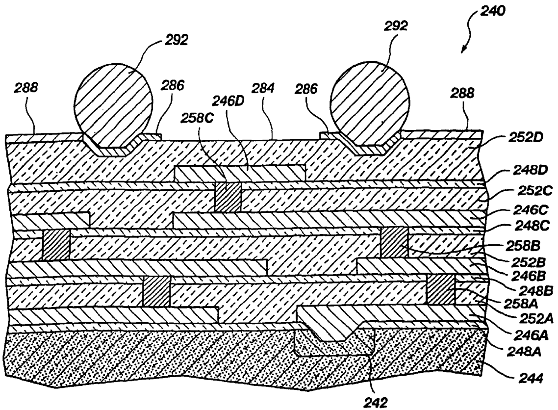
Fig. 11 (PRIOR ART)
