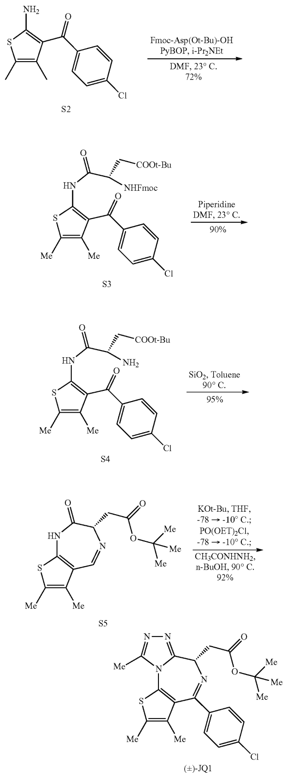
Scheme S2. Synthesis of enantiomerically enriched ( \pm )-JQ1.
