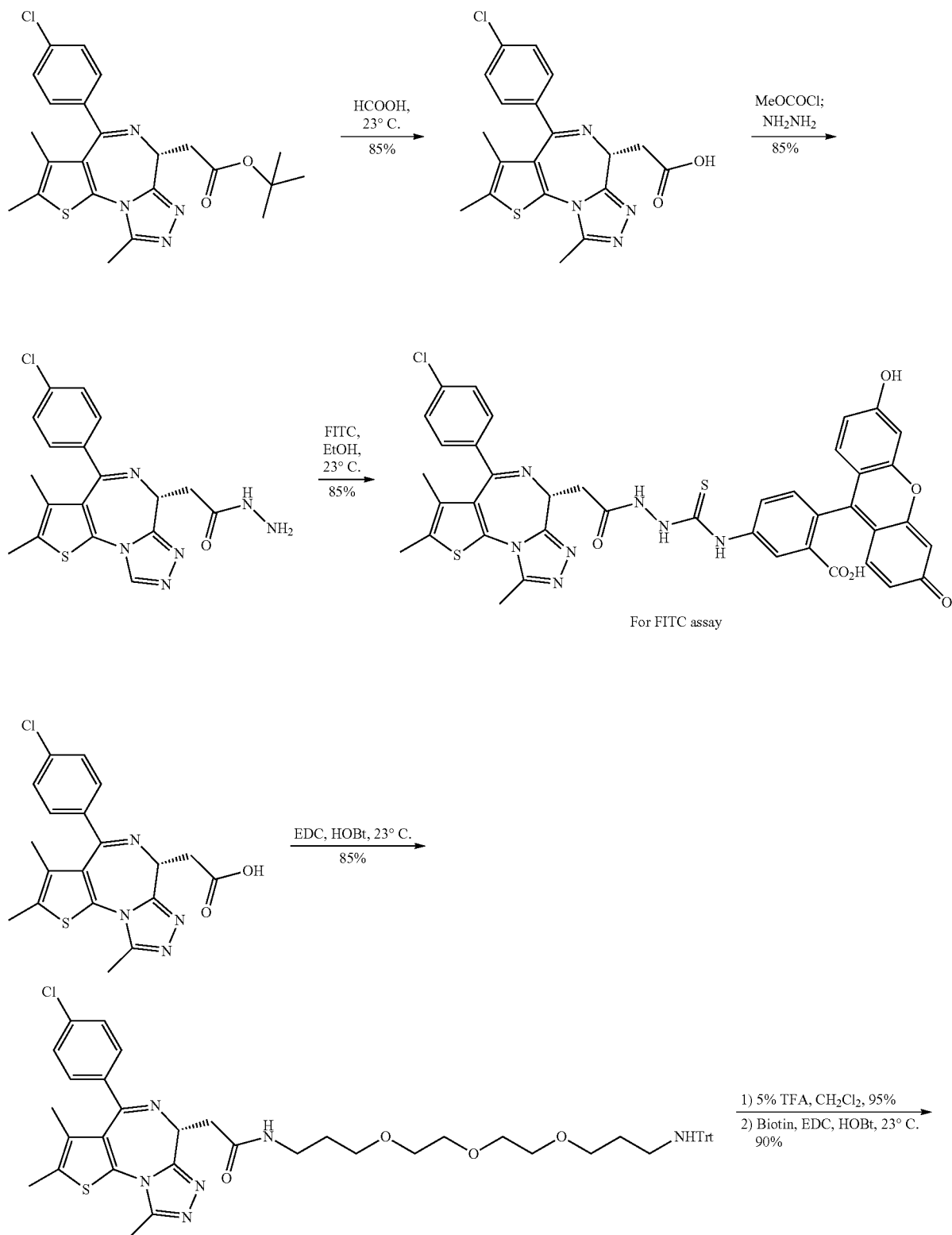
Scheme S4. Synthesis of derivatives useful as probes.
