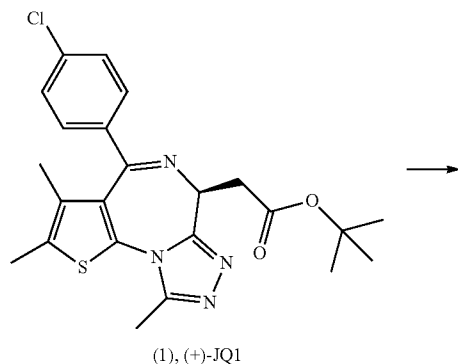
Scheme S3. Synthesis of hydrazine derivatives.
