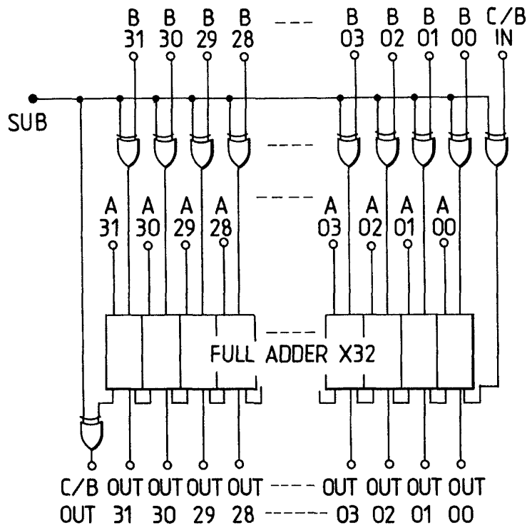
(a) ARITHMETIC LOGIC OPERATION CIRCUIT
