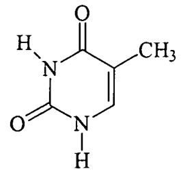
Thymine
