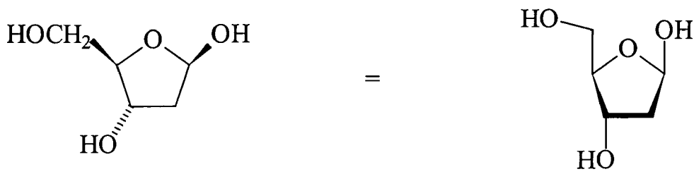
β-D-2-Deoxyribose
