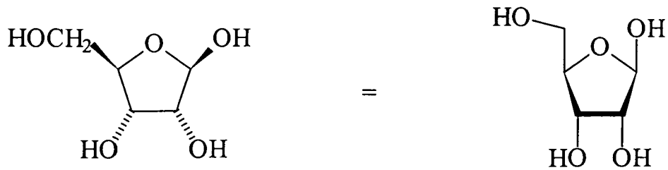
β-D-Ribose
