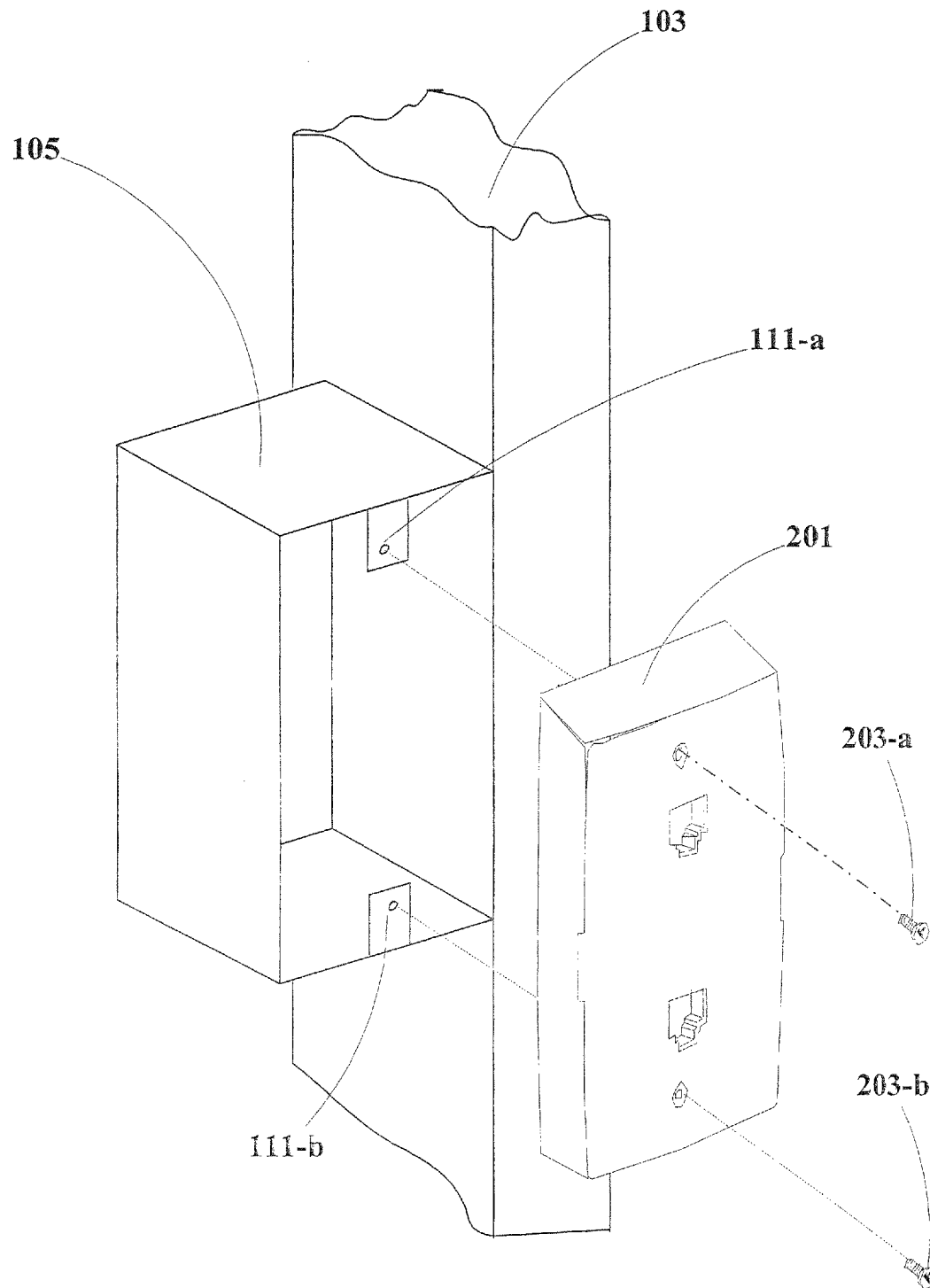
FIG. 2 (PRIOR ART)
