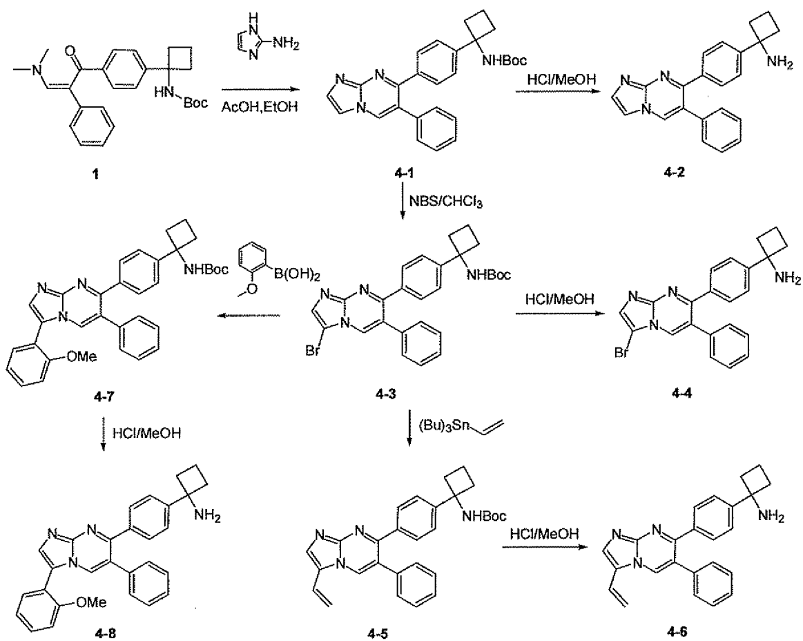
Reaction Scheme 4
