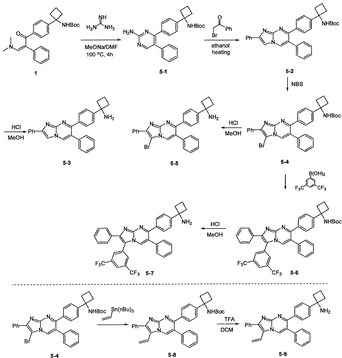
Reaction Scheme 5
