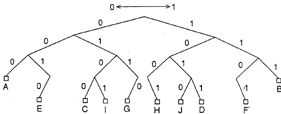
DECODING TREE IN ORDER DIRECTION
