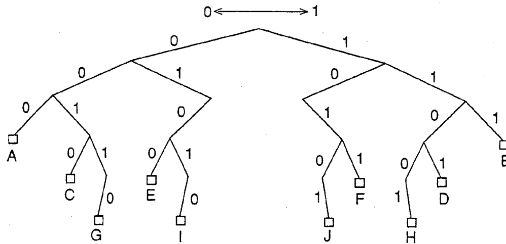
DECODING TREE IN REVERSE DIRECTION
