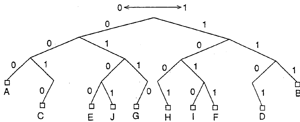
DECODING TREE IN REVERSE DIRECTION
