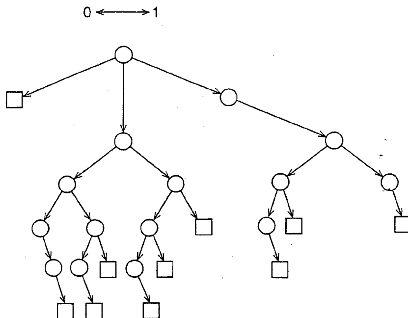
DECODING TREE
