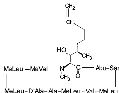
Z-isomer
